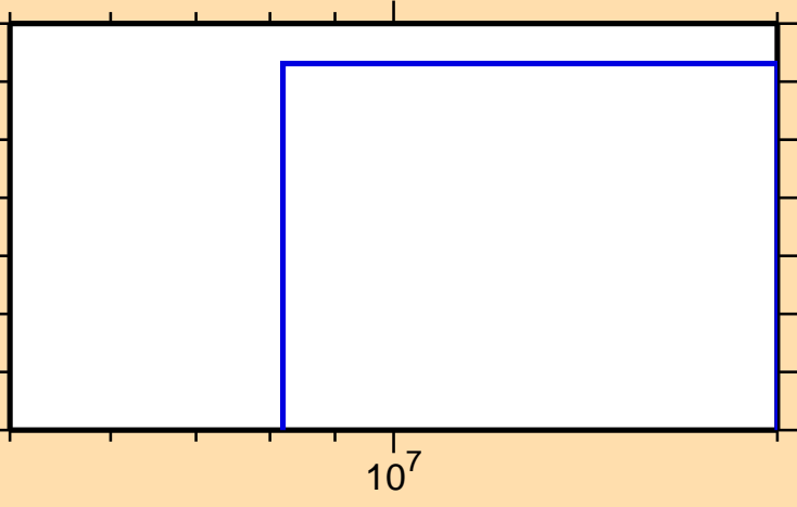
\sigma vs. E for ^{232}\text{Am}(n,2n\alpha)
