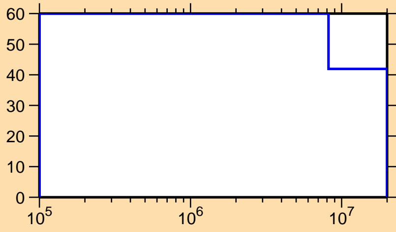
\Delta\sigma/\sigma vs. E for ^{232}\text{Am}(n,n_1)
