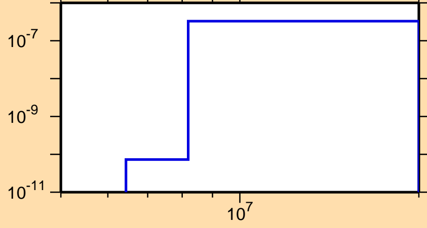
\sigma vs. E for ^{232}\text{Am}(n,t)
