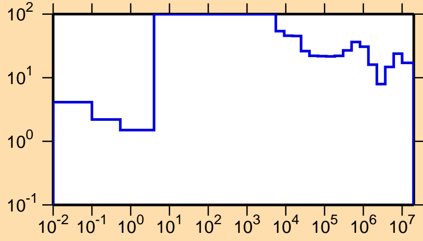
\Delta\sigma/\sigma vs. E for ^{233}\text{Am}(n,\text{tot.})
