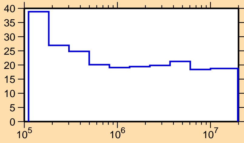
\Delta\sigma/\sigma vs. E for ^{233}\text{Am}(n,\text{nonel.})
