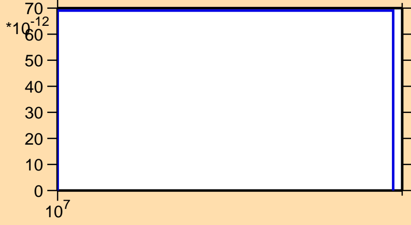
\sigma vs. E for ^{233}\text{Am} (mt 45)
