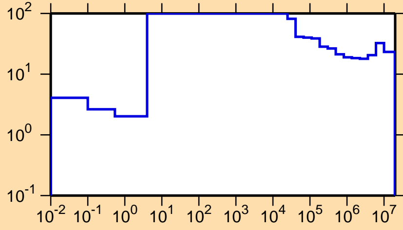
\Delta\sigma/\sigma vs. E for ^{233}\text{Am}(n,f)
