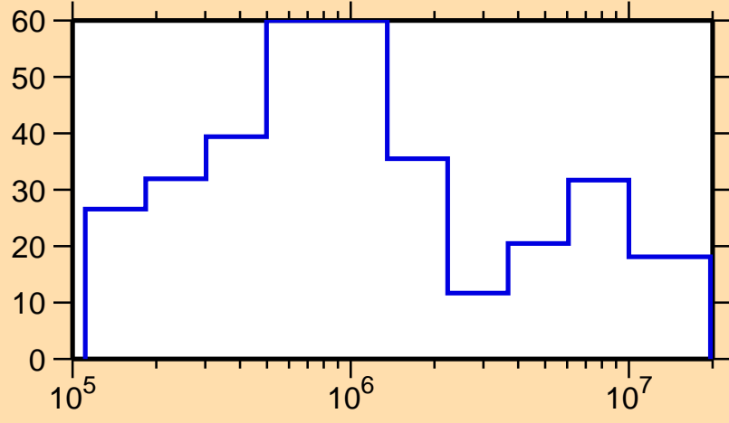
\Delta\sigma/\sigma vs. E for ^{233}\text{Am}(n,\text{el.})
