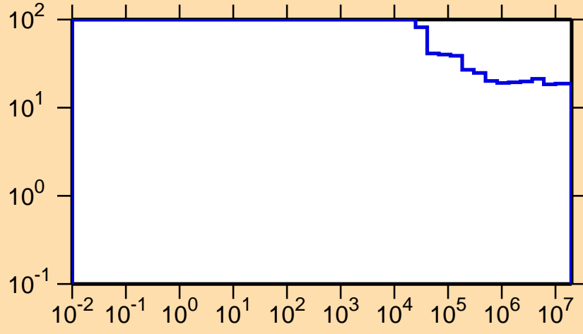
\Delta\sigma/\sigma vs. E for ^{233}\text{Am}(n,\text{nonel.})
