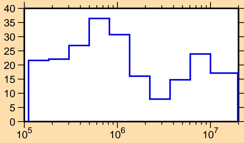
\Delta\sigma/\sigma vs. E for ^{233}\text{Am}(n, \text{tot.})
