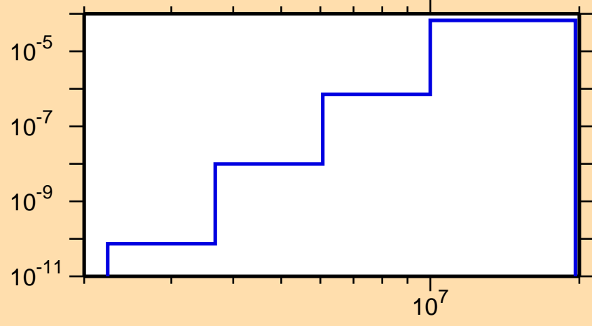
\sigma vs. E for ^{233}\text{Am}(n,\alpha)
