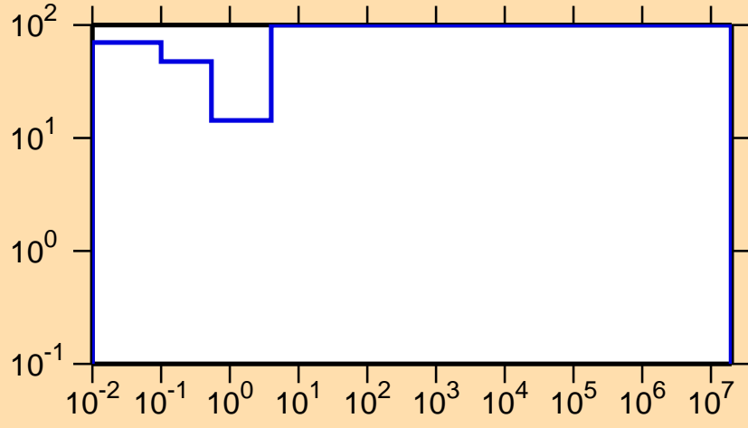
\Delta\sigma/\sigma vs. E for ^{233}\text{Am}(n,\gamma)
