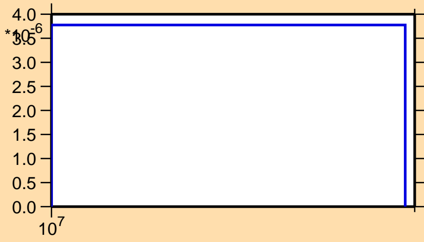
\sigma vs. E for ^{233}\text{Am}(n,\text{nd})
