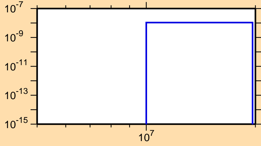
\sigma vs. E for ^{233}\text{Am}(n,\text{He3})
