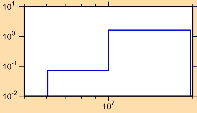
\sigma vs. E for ^{233}\text{Am}(n,2n)
