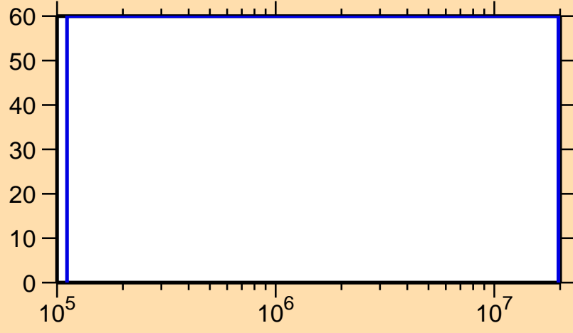
\Delta\sigma/\sigma vs. E for ^{233}\text{Am}(n,\text{inel.})
