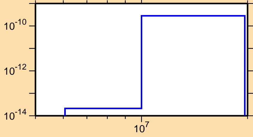
\sigma vs. E for ^{233}\text{Am}(n, p\alpha)
