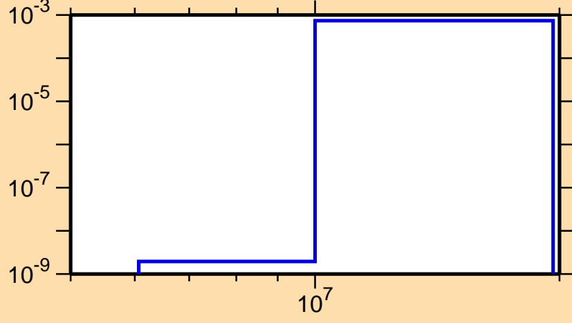
\sigma vs. E for ^{233}\text{Am}(n,t)
