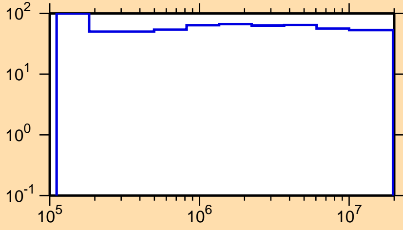
\Delta\sigma/\sigma vs. E for ^{233}\text{Am}(n,n_1)
