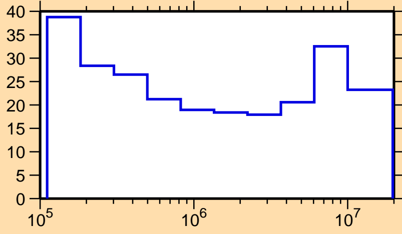
\Delta\sigma/\sigma vs. E for ^{233}\text{Am}(n,f)
