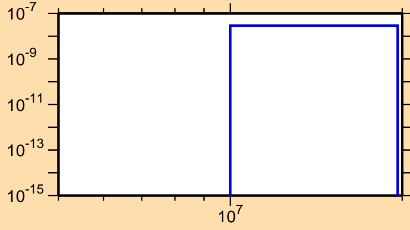
\sigma vs. E for ^{233}\text{Am}(n,2n\alpha)
