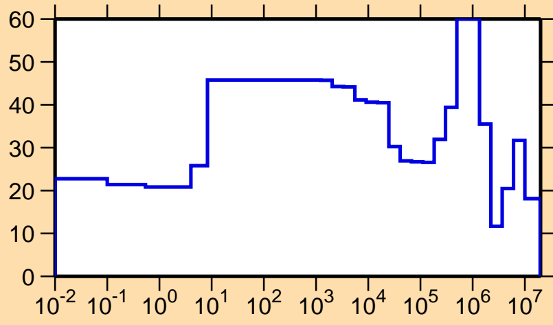
\Delta\sigma/\sigma vs. E for ^{233}\text{Am}(n,\text{el.})
