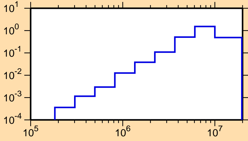
\sigma vs. E for ^{233}\text{Am}(n,n\text{cont.})
