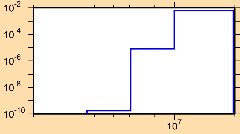
\sigma vs. E for ^{233}\text{Am}(n,d)
