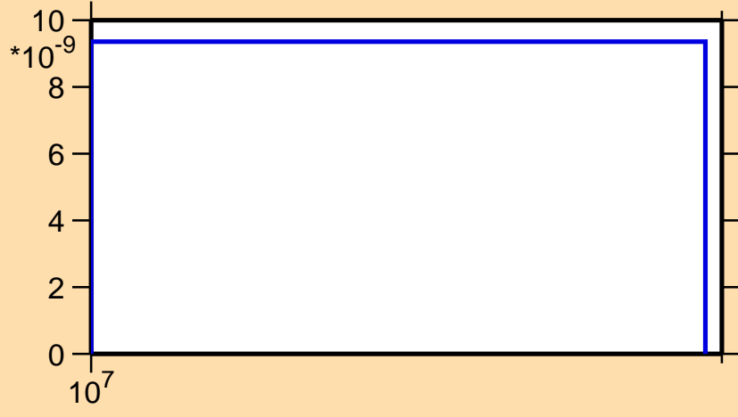
\sigma vs. E for ^{233}\text{Am}(n,nt)
