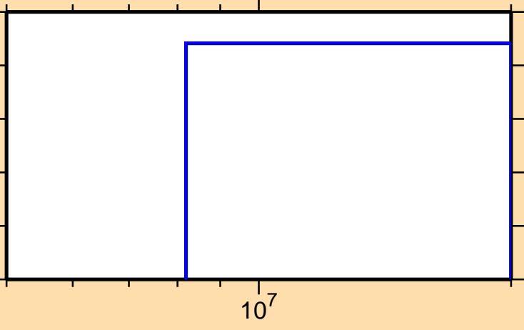
\sigma vs. E for ^{233}\text{Am}(n,\text{He3})
