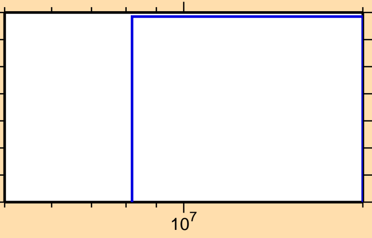
\sigma vs. E for ^{233}\text{Am}(n,3n)
