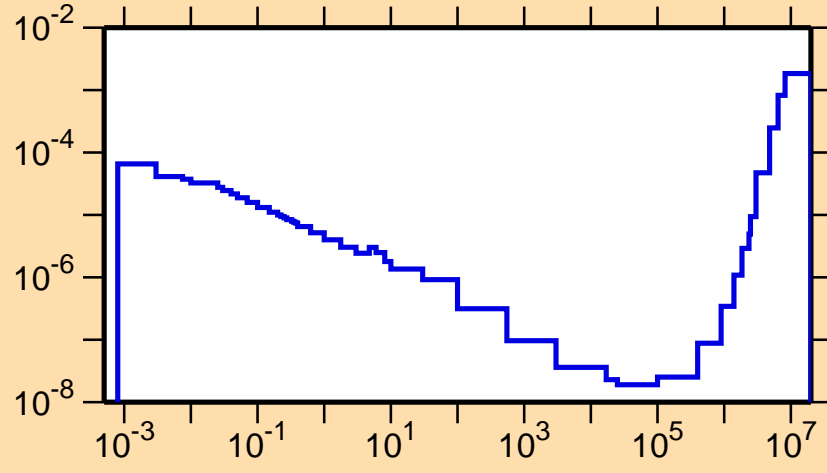
\sigma vs. E for ^{233}\text{Am}(n,p)
