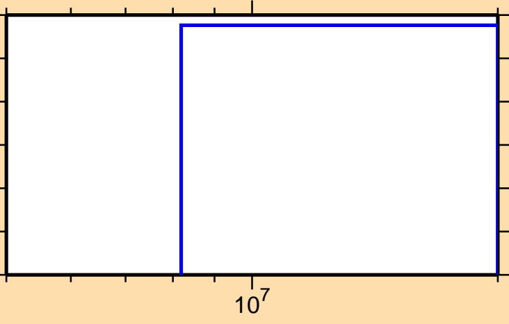
\sigma vs. E for ^{233}\text{Am} (mt 45)
