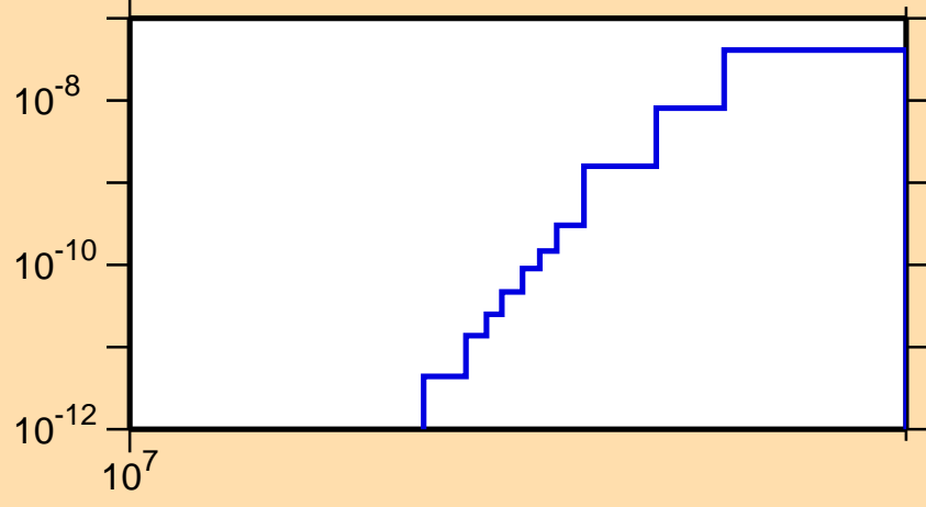
\sigma vs. E for ^{234}\text{Am}(n,\text{nd})
