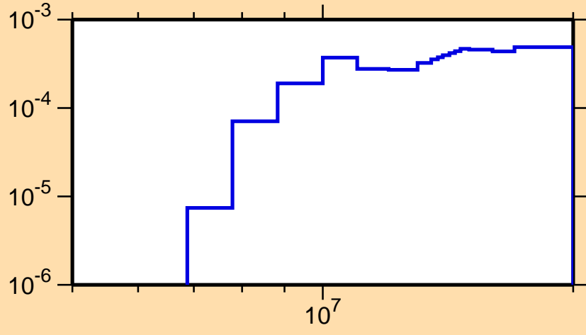
\sigma vs. E for ^{234}\text{Am}(n,2n)
