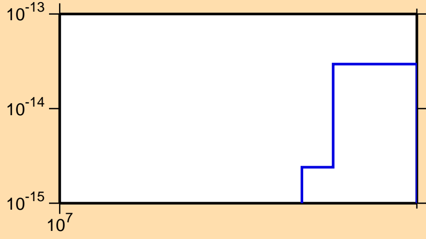
\sigma vs. E for ^{234}\text{Am} (mt 45)
