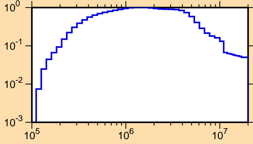
\sigma vs. E for ^{234}\text{Am}(n,\text{inel.})
