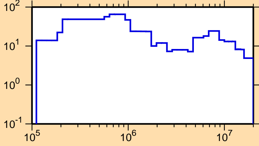
\Delta\sigma/\sigma vs. E for ^{234}\text{Am}(n,\text{el.})
