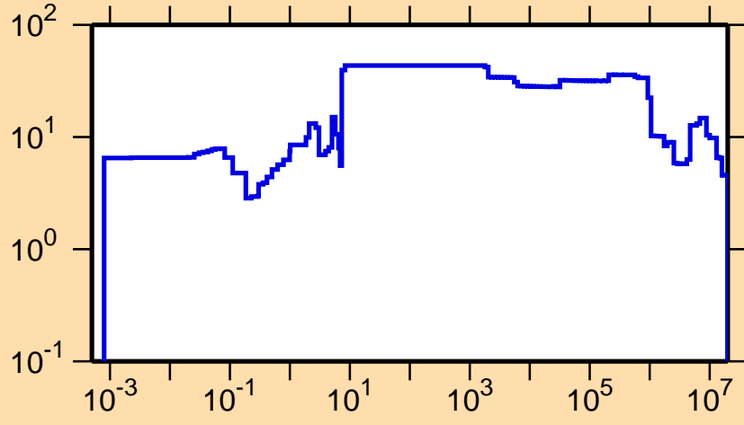
\Delta\sigma/\sigma vs. E for ^{234}\text{Am}(n,\text{tot.})
