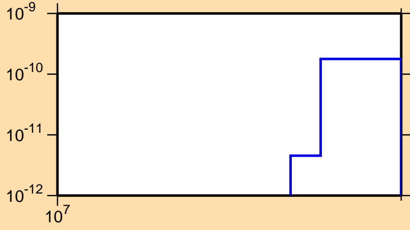
\sigma vs. E for ^{234}\text{Am}(n,nt)
