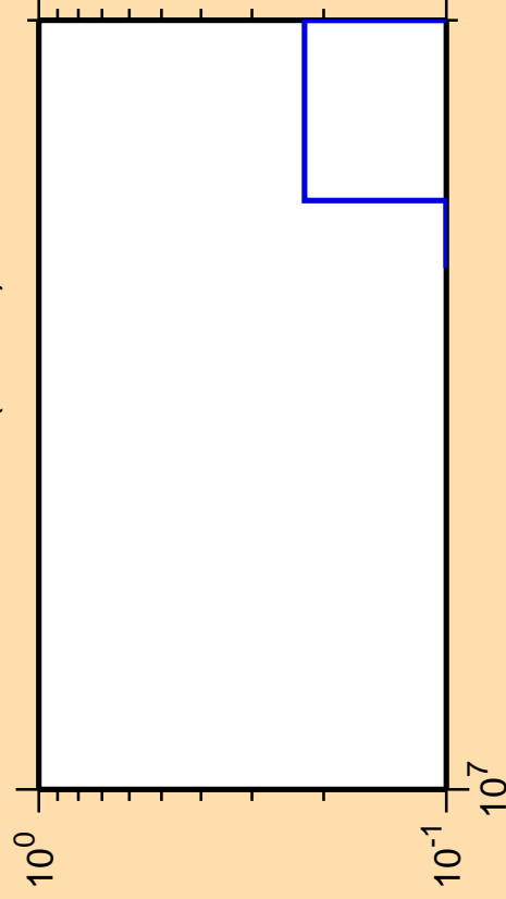
\Delta\sigma/\sigma vs. E for ^{234}\text{Am} (mt 45)
