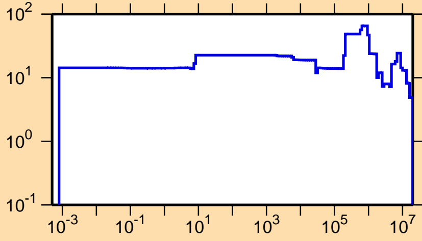
\Delta\sigma/\sigma vs. E for ^{234}\text{Am}(n,el.)
