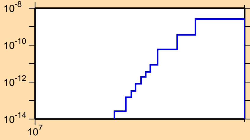
\sigma vs. E for ^{234}\text{Am}(n,2np)
