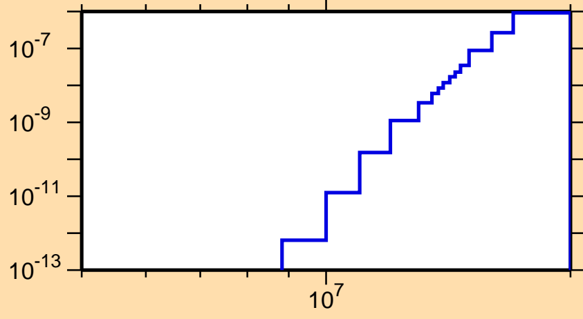
\sigma vs. E for ^{234}\text{Am}(n,\text{He3})
