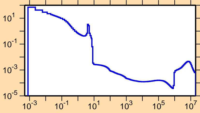
\sigma vs. E for ^{234}\text{Am}(n,\gamma)
