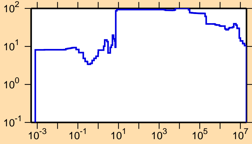
\Delta\sigma/\sigma vs. E for ^{234}\text{Am}(n,f)
