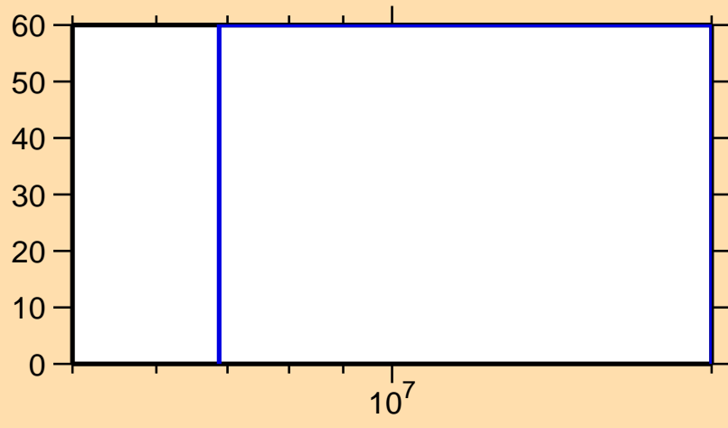
\Delta\sigma/\sigma vs. E for ^{234}\text{Am}(n,2n)
