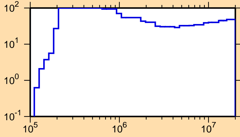
\Delta\sigma/\sigma vs. E for ^{234}\text{Am}(n,n_1)
