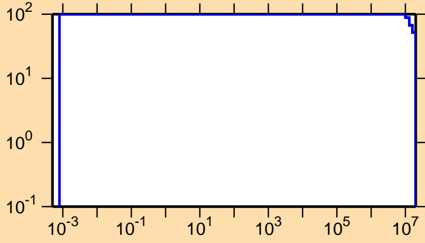
\Delta\sigma/\sigma vs. E for ^{234}\text{Am}(n,p)
