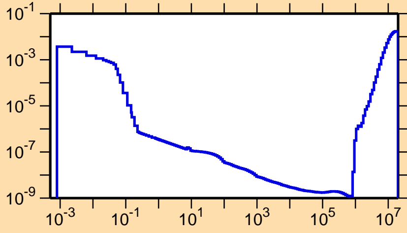
\sigma vs. E for ^{234}\text{Am}(n,p)
