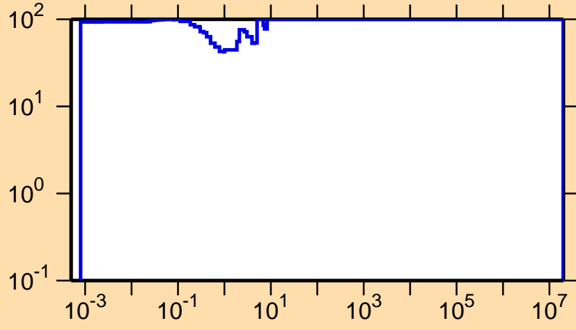
\Delta\sigma/\sigma vs. E for ^{234}\text{Am}(n,\gamma)
