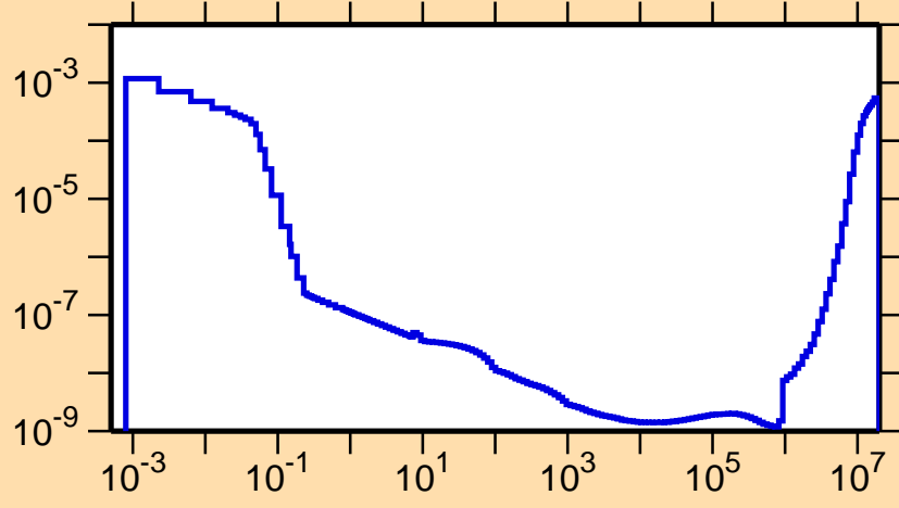
\sigma vs. E for ^{234}\text{Am}(n,\alpha)
