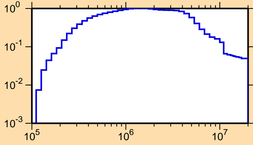
\sigma vs. E for ^{234}\text{Am}(n,n\text{cont.})
