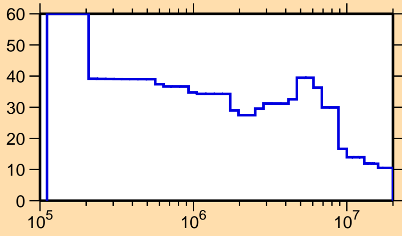
\Delta\sigma/\sigma vs. E for ^{234}\text{Am}(n,f)
