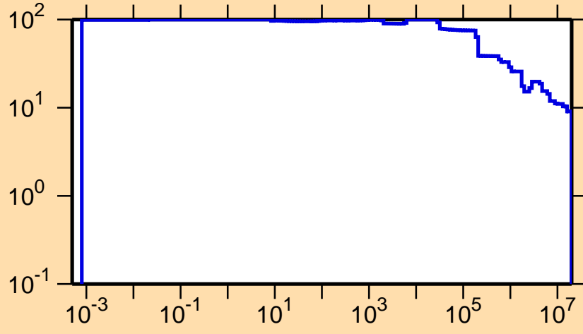
\Delta\sigma/\sigma vs. E for ^{234}\text{Am}(n,\text{nonel.})
