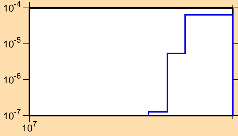
\sigma vs. E for ^{234}\text{Am}(n,3n)
