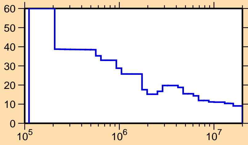
\Delta\sigma/\sigma vs. E for ^{234}\text{Am}(n,\text{nonel.})
