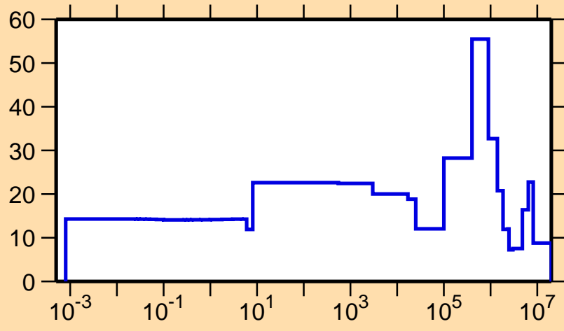
\Delta\sigma/\sigma vs. E for ^{234}\text{Am}(n,el.)
