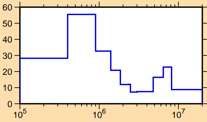
\Delta\sigma/\sigma vs. E for ^{234}\text{Am}(n,\text{el.})
