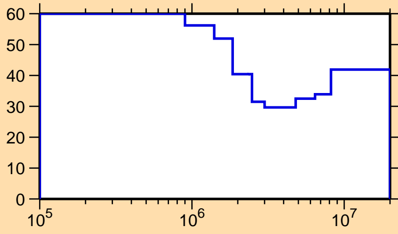
\Delta\sigma/\sigma vs. E for ^{234}\text{Am}(n,n_1)
