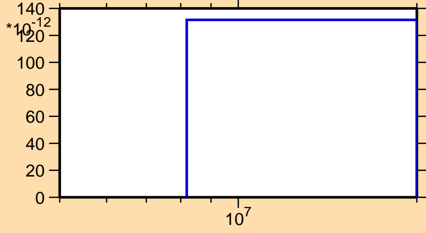
\sigma vs. E for ^{234}\text{Am}(n,2n\alpha)
