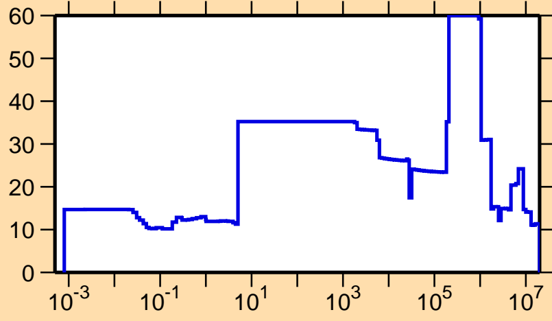
\Delta\sigma/\sigma vs. E for ^{235}\text{Am}(n,el.)
