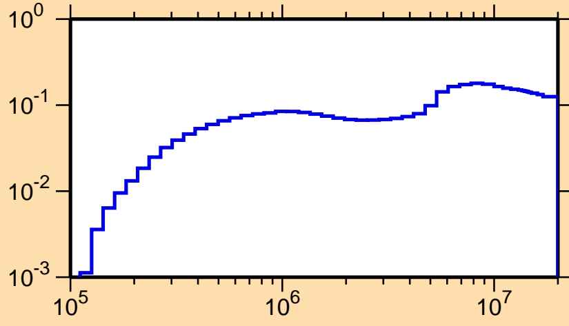
\sigma vs. E for ^{235}\text{Am}(n,\text{inel.})
