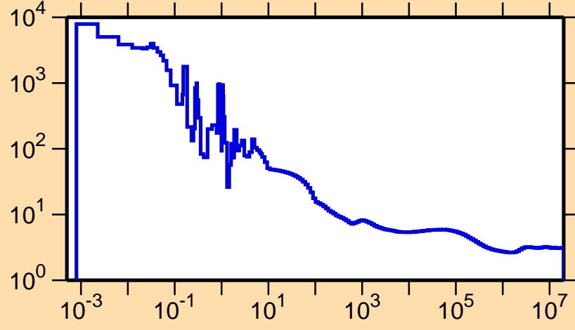
\sigma vs. E for ^{235}\text{Am}(n,f)
