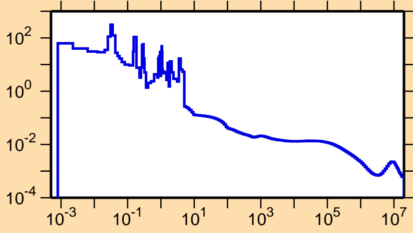
\sigma vs. E for ^{235}\text{Am}(n,\gamma)
