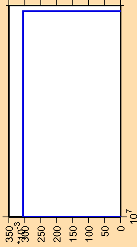
\Delta\sigma/\sigma vs. E for ^{235}\text{Am} (mt 45)
