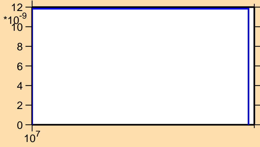
\sigma vs. E for ^{235}\text{Am}(n,\text{nd})
