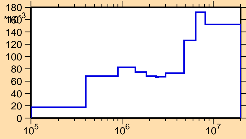
\sigma vs. E for ^{235}\text{Am}(n,n\text{cont.})
