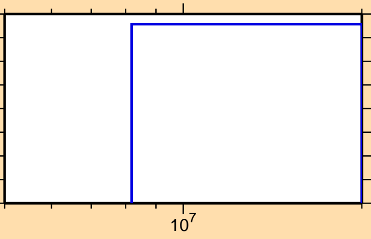
\sigma vs. E for ^{235}\text{Am} (mt 45)
