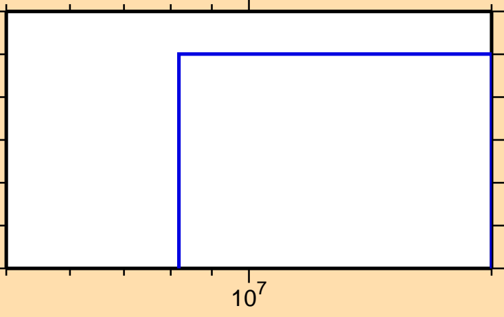
\sigma vs. E for ^{235}\text{Am}(n,\text{nd})
