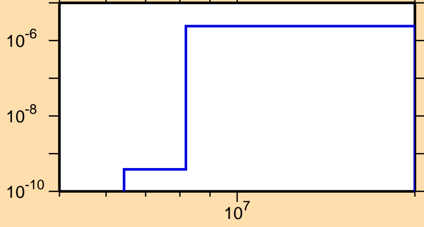
\sigma vs. E for ^{235}\text{Am}(n,np)
