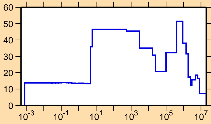
\Delta\sigma/\sigma vs. E for ^{236}\text{Am}(n,el.)
