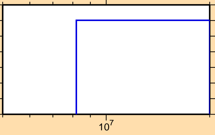
\sigma vs. E for ^{236}\text{Am}(n,2n\alpha)
