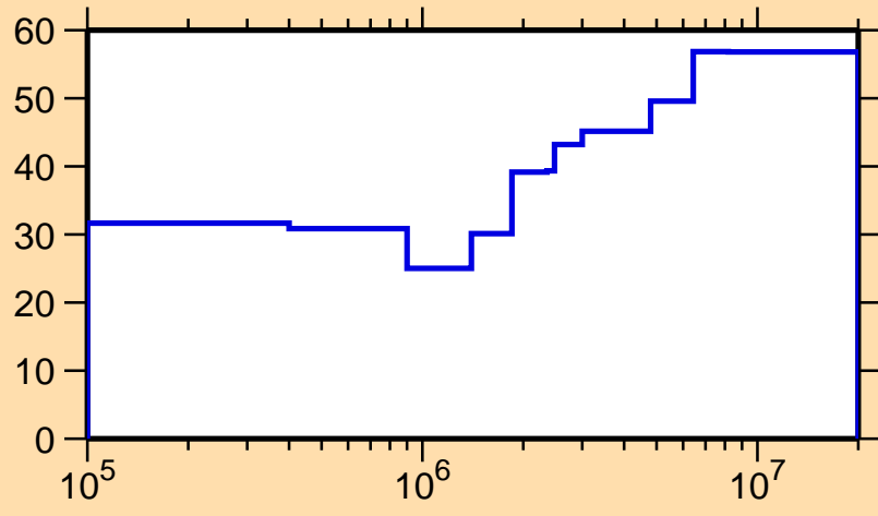
\Delta\sigma/\sigma vs. E for ^{236}\text{Am}(n,n_1)
