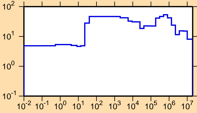
\Delta\sigma/\sigma vs. E for ^{236}\text{Am}(n,el.)
