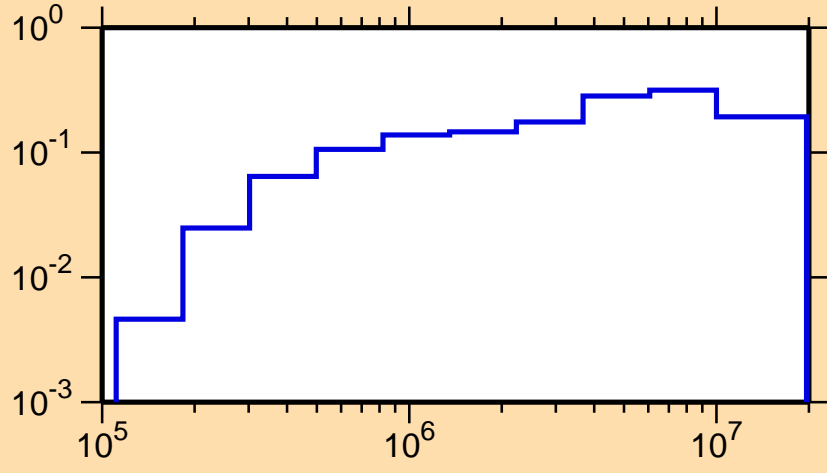
\sigma vs. E for ^{236}\text{Am}(n,n\text{cont.})
