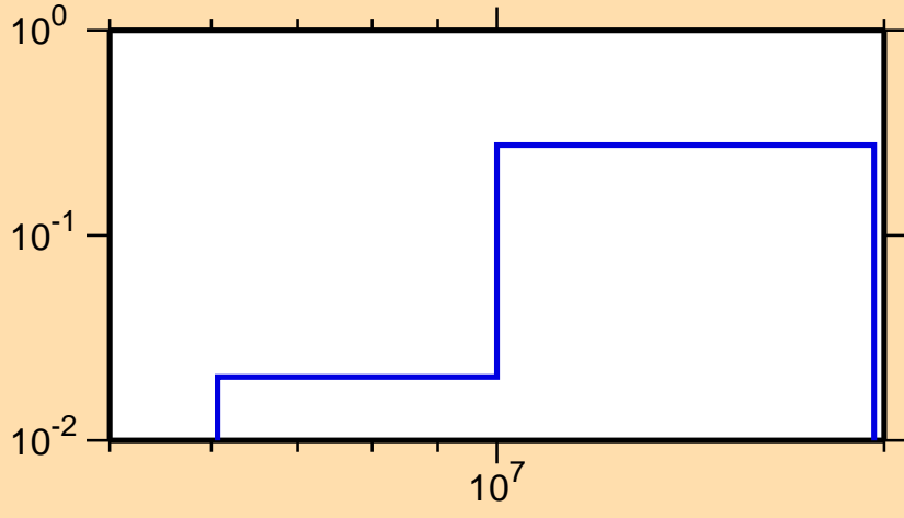
\sigma vs. E for ^{236}\text{Am}(n,2n)
