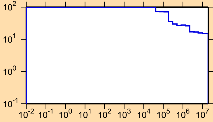
\Delta\sigma/\sigma vs. E for ^{236}\text{Am}(n,\text{nonel.})
