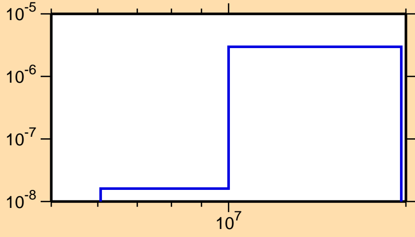
\sigma vs. E for ^{236}\text{Am}(n,np)
