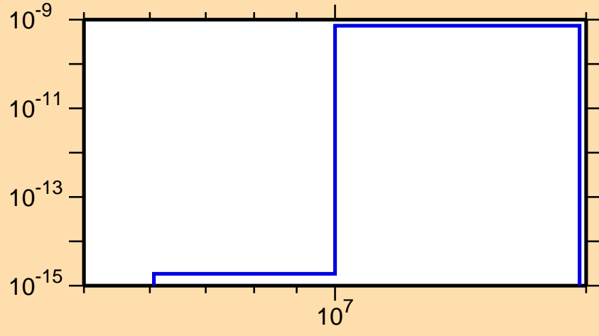
\sigma vs. E for ^{236}\text{Am}(n,\text{He3})
