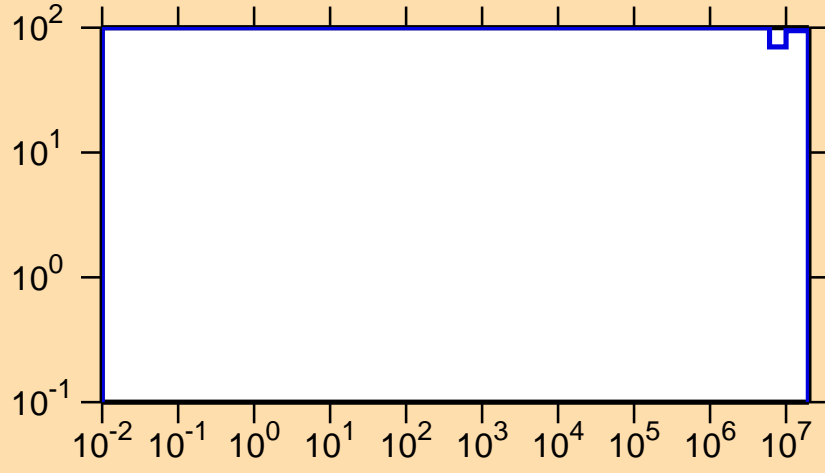
\Delta\sigma/\sigma vs. E for ^{236}\text{Am}(n,p)
