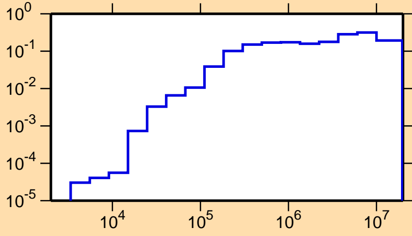
\sigma vs. E for ^{236}\text{Am}(n,\text{inel.})
