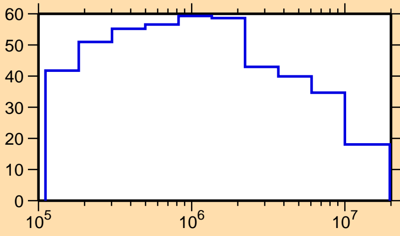
\Delta\sigma/\sigma vs. E for ^{236}\text{Am}(n,f)
