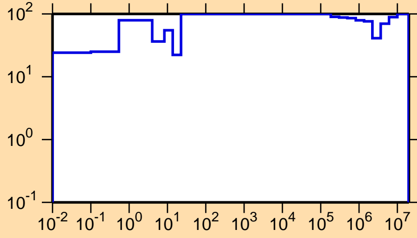
\Delta\sigma/\sigma vs. E for ^{236}\text{Am}(n,\gamma)
