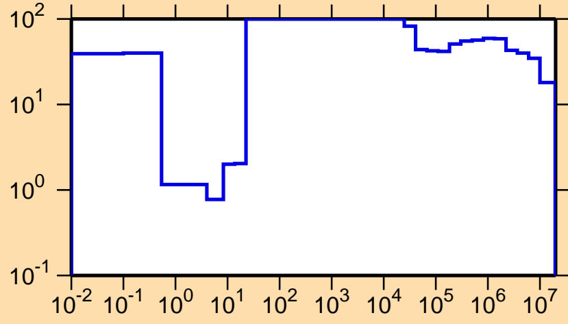
\Delta\sigma/\sigma vs. E for ^{236}\text{Am}(n,f)
