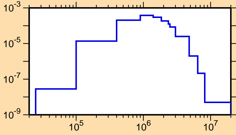
\sigma vs. E for ^{236}\text{Am}(n,n_2)
