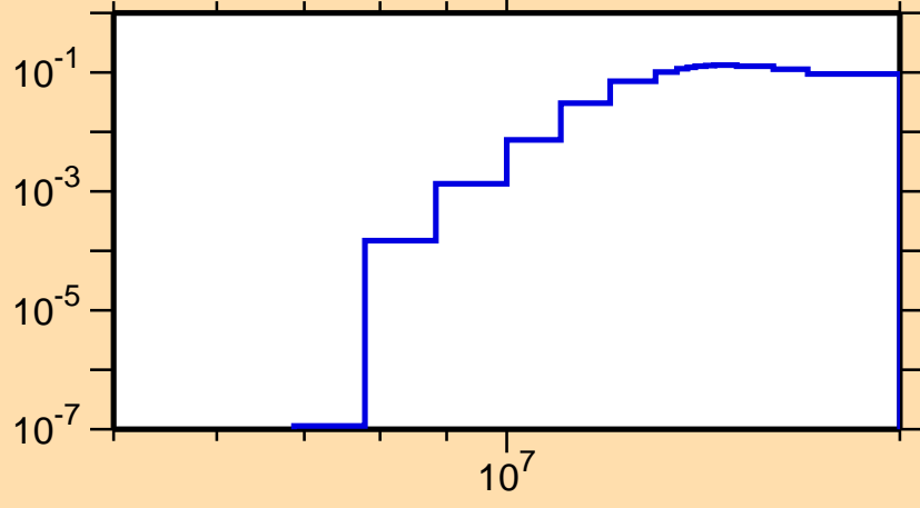
\sigma vs. E for ^{237}\text{Am}(n,2n)
