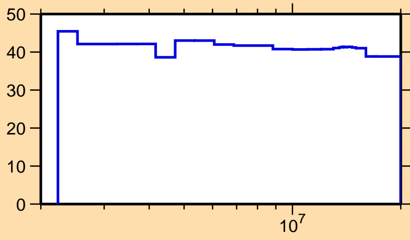
\Delta\sigma/\sigma vs. E for ^{237}\text{Am}(n,n_1)
