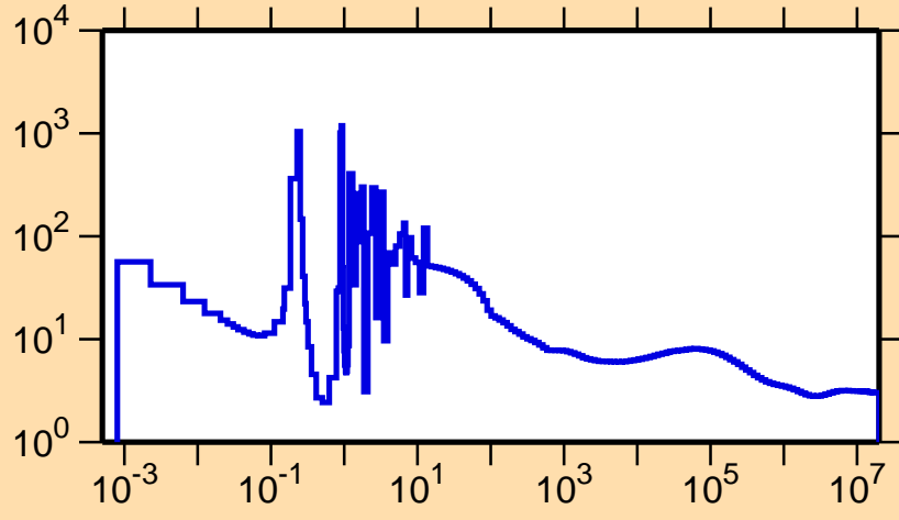
\sigma vs. E for ^{237}\text{Am}(n,\text{nonel.})
