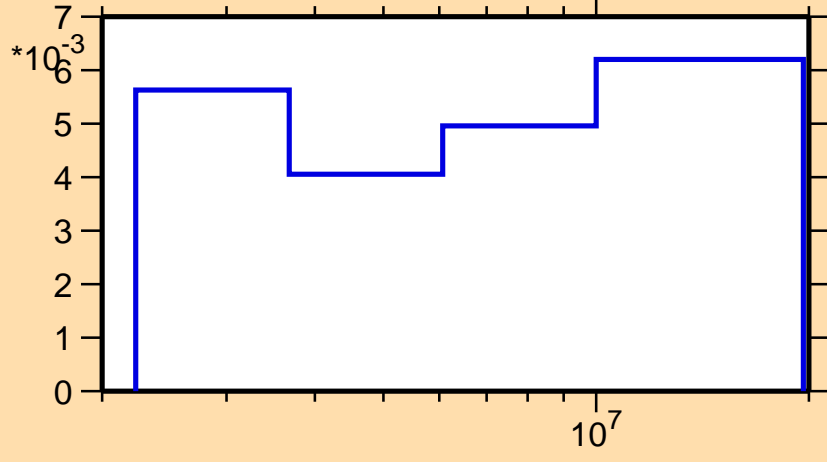
\sigma vs. E for ^{237}\text{Am}(n,n\text{cont.})
