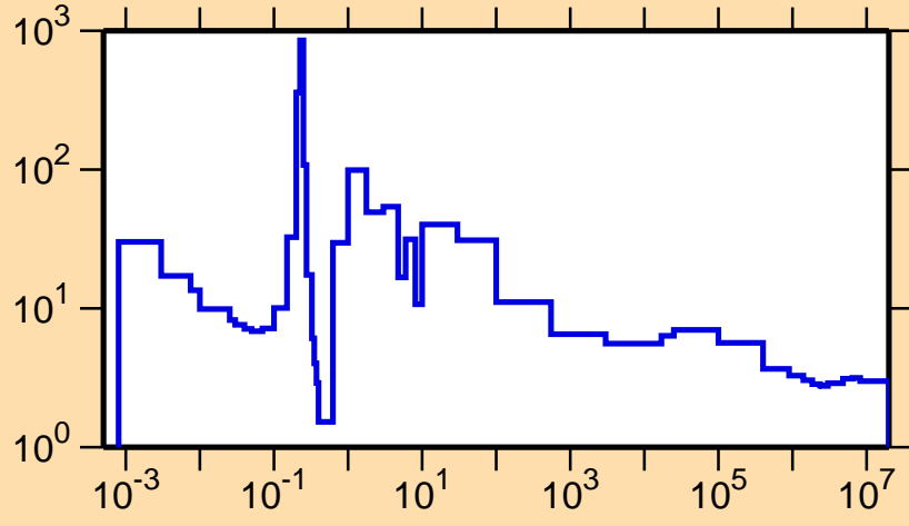
\sigma vs. E for ^{237}\text{Am}(n,f)
