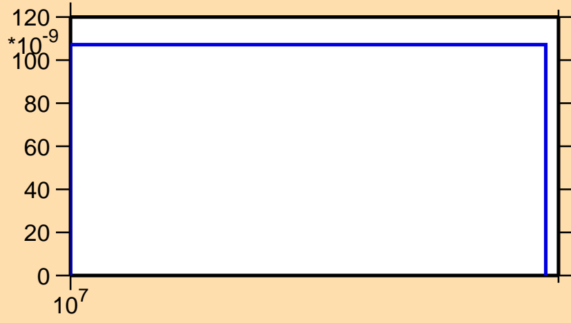
\sigma vs. E for ^{238}\text{Am}(n,\text{nd})
