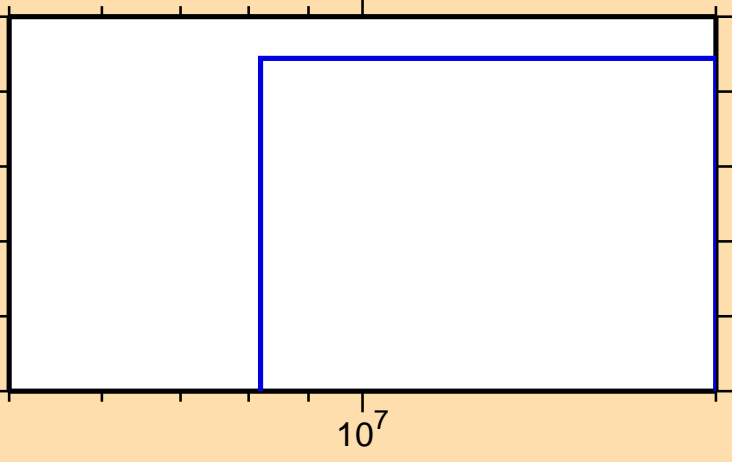
\sigma vs. E for ^{238}\text{Am}(n,\text{nd})
