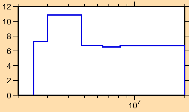
\Delta\sigma/\sigma vs. E for ^{238}\text{Am}(n,\text{nonel.})
