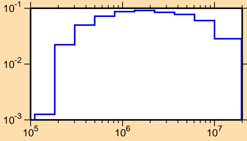
\sigma vs. E for ^{239}\text{Am}(n,n_3)
