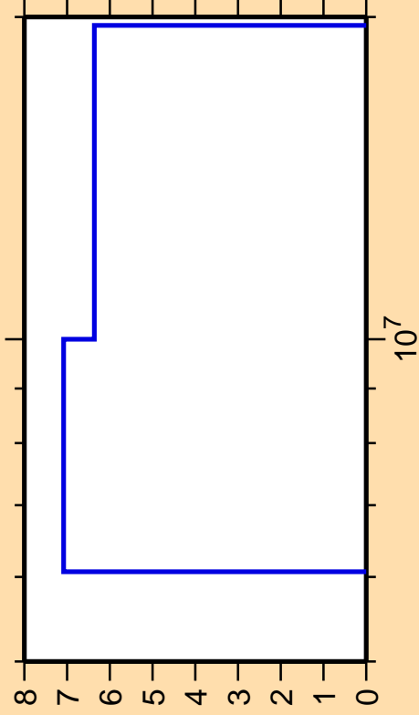
\Delta\sigma/\sigma vs. E for ^{239}\text{Am}(n,np)
