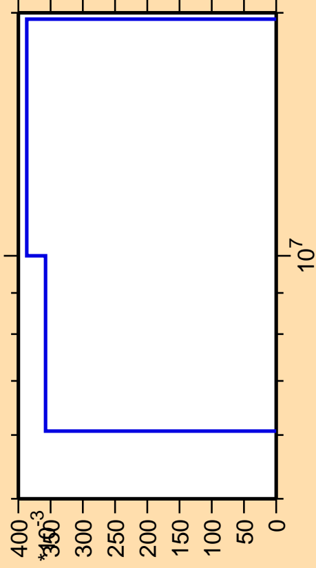
\Delta\sigma/\sigma vs. E for ^{239}\text{Am}(n,f)
