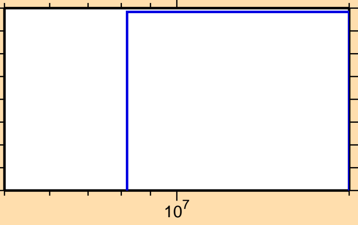
\sigma vs. E for ^{239}\text{Am}(n,\text{He3})
