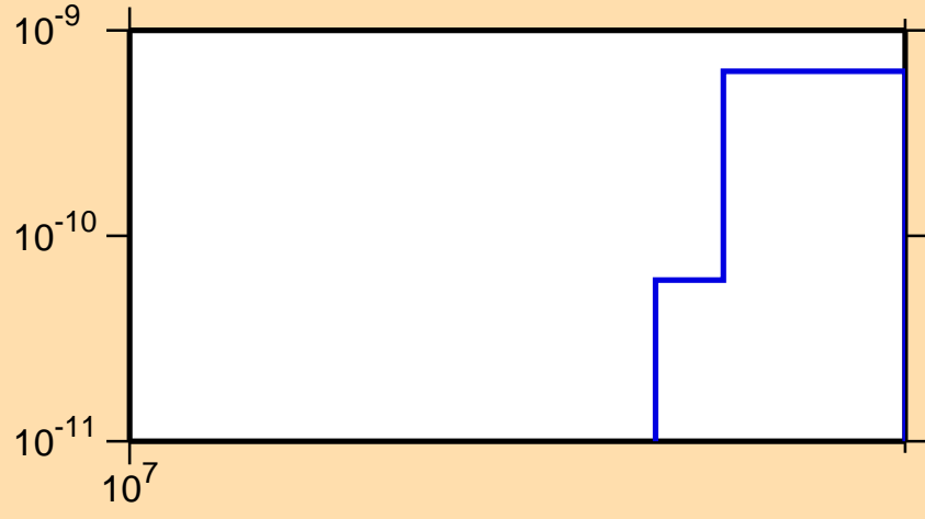
\sigma vs. E for ^{240}\text{Am}(n,3n\alpha)
