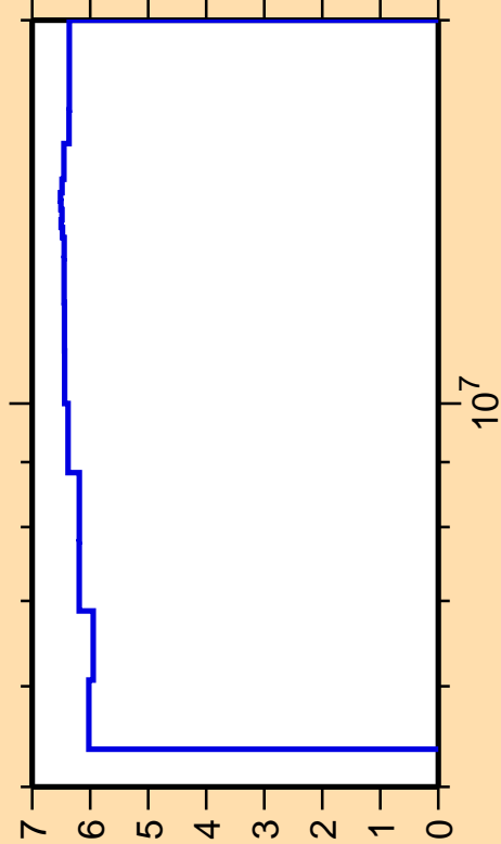
\Delta\sigma/\sigma vs. E for ^{240}\text{Am}(n,\gamma)
