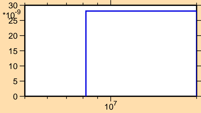
\sigma vs. E for ^{240}\text{Am}(n,2n\alpha)
