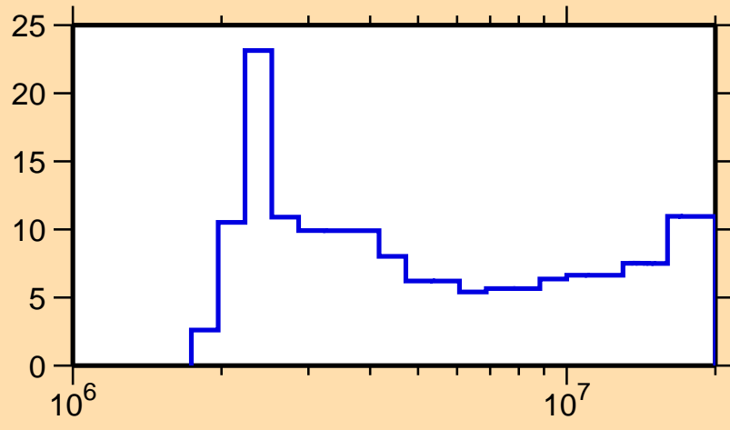
\Delta\sigma/\sigma vs. E for ^{242}\text{Am}(n,p)
