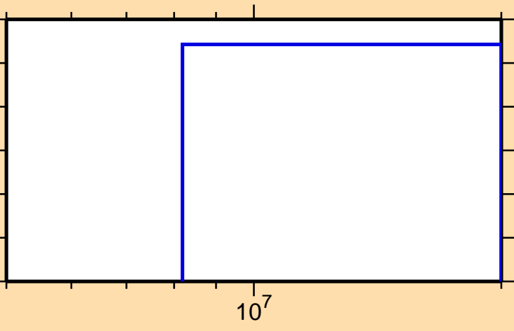
\sigma vs. E for ^{242}\text{Am}(n,2np)
