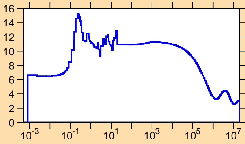
\sigma vs. E for ^{242}\text{Am}(n,\text{el.})
