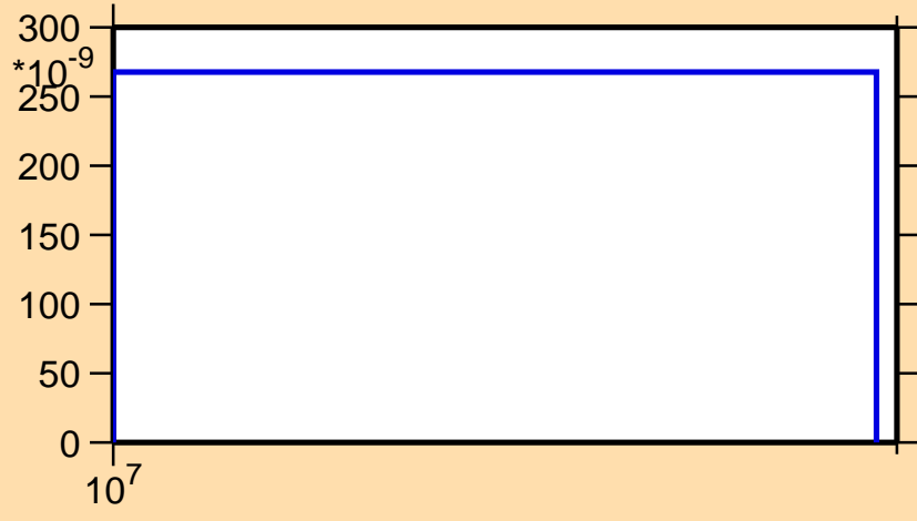
\sigma vs. E for ^{242}\text{Am}(n,\text{nd})
