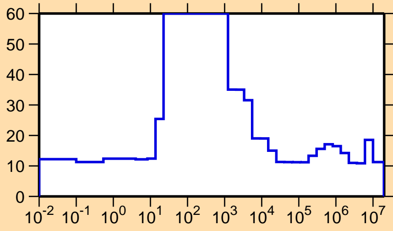
\Delta\sigma/\sigma vs. E for ^{242}\text{Am}(n,el.)
