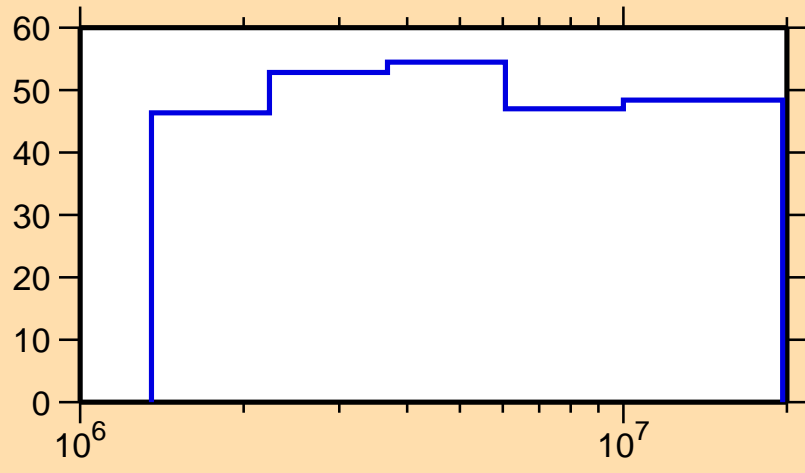
\Delta\sigma/\sigma vs. E for ^{242}\text{Am}(n,ncont.)
