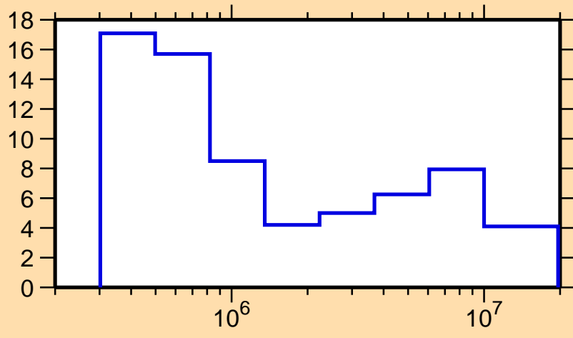
\Delta\sigma/\sigma vs. E for ^{242}\text{Am}(n,\text{tot.})
