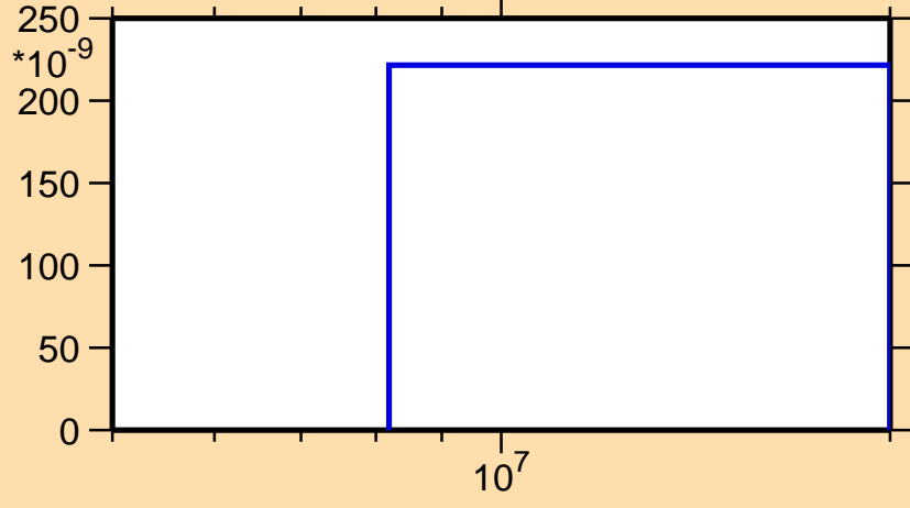
\sigma vs. E for ^{242}\text{Am}(n,nd)
