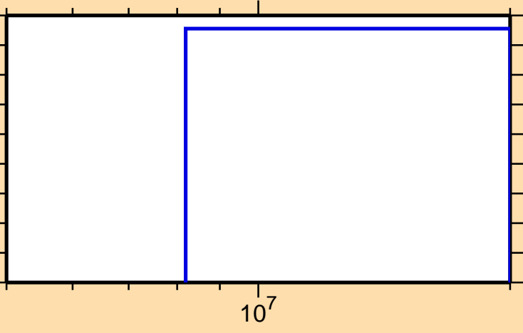
\sigma vs. E for ^{242}\text{Am}(n,3n\alpha)
