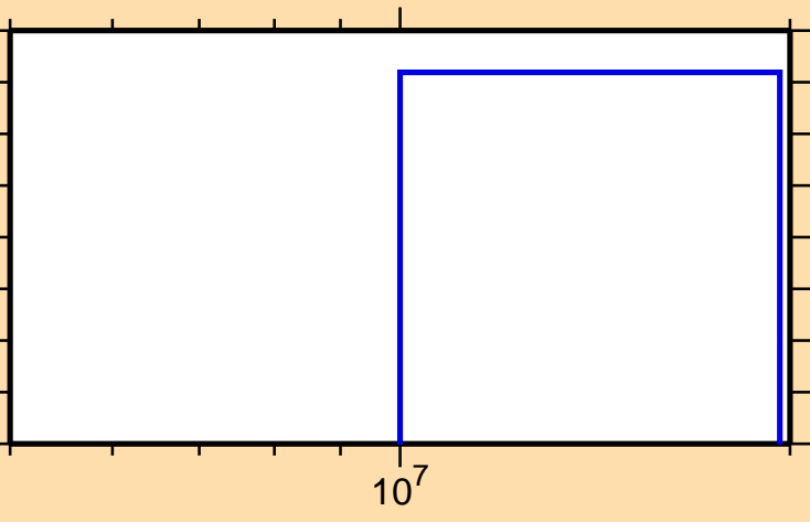
\sigma vs. E for ^{243}\text{Am}(n,2n\alpha)
