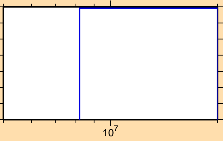
\sigma vs. E for ^{243}\text{Am}(n,\text{nd})
