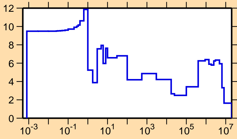
\Delta\sigma/\sigma vs. E for ^{243}\text{Am}(n,el.)
