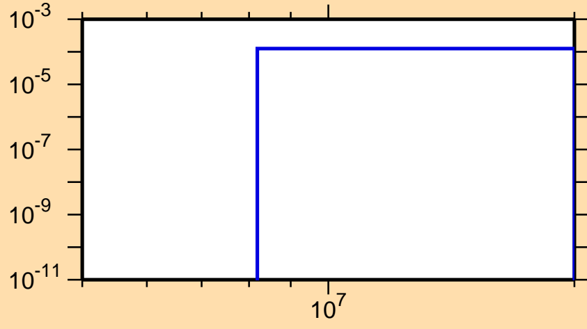
\sigma vs. E for ^{243}\text{Am}(n,np)
