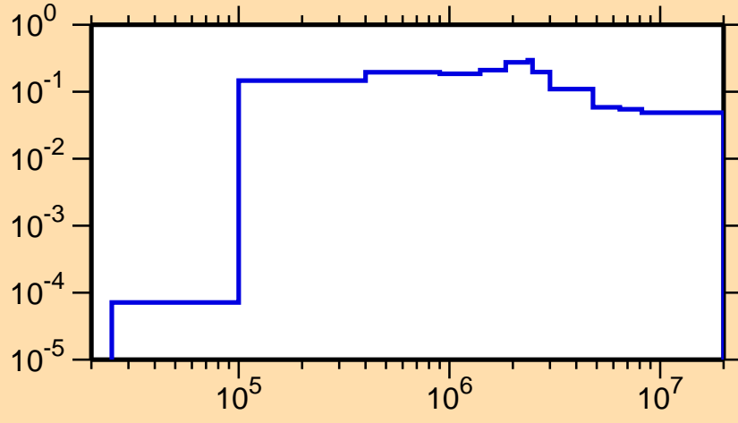
\sigma vs. E for ^{243}\text{Am}(n,n_3)
