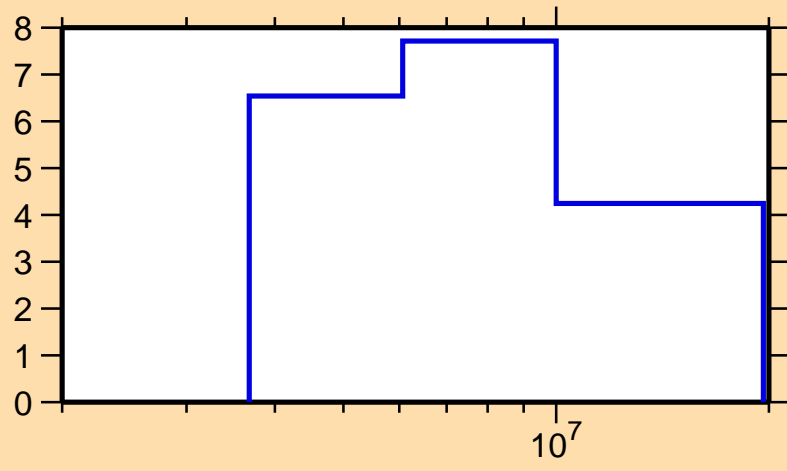
\Delta\sigma/\sigma vs. E for ^{244}\text{Am}(n,\text{el.})
