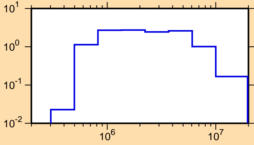
\sigma vs. E for ^{244}\text{Am}(n,n\text{cont.})
