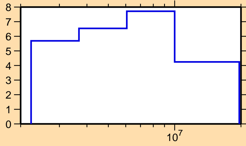
\Delta\sigma/\sigma vs. E for ^{244}\text{Am}(n,el.)
