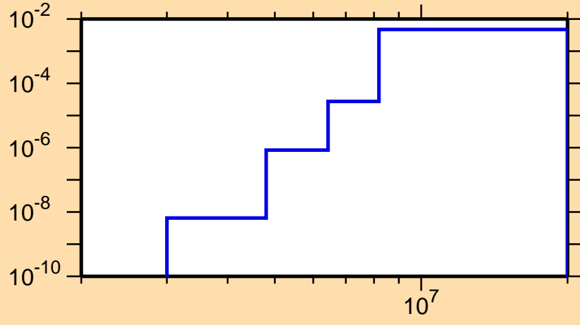
\sigma vs. E for ^{244}\text{Am}(n,p)
