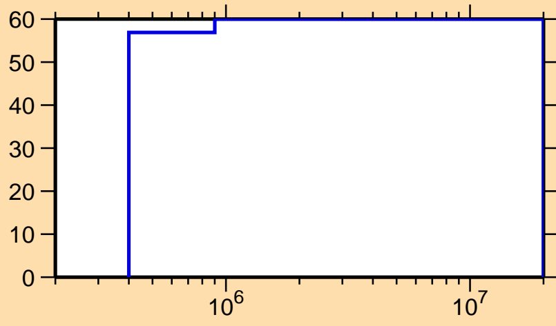
\Delta\sigma/\sigma vs. E for ^{244}\text{Am}(n,n_1)
