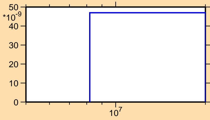
\sigma vs. E for ^{244}\text{Am}(n,nt)
