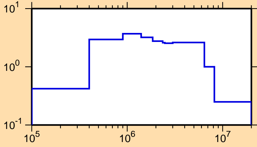
\sigma vs. E for ^{244}\text{Am}(n,\text{inel.})
