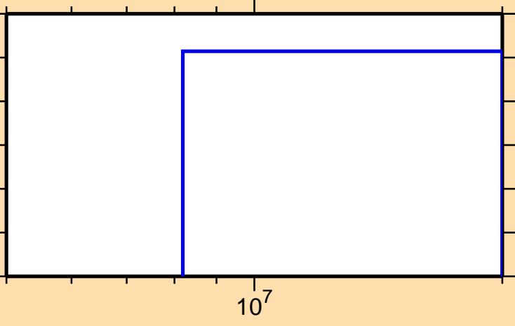
\sigma vs. E for ^{244}\text{Am}(n,2n\alpha)
