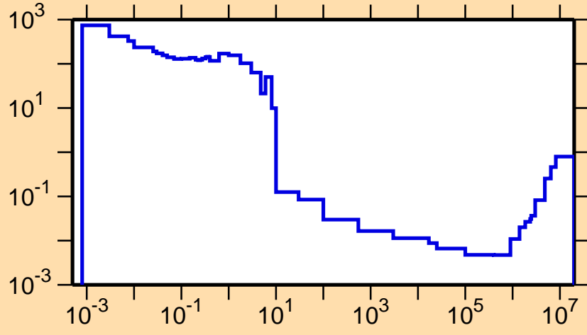
\sigma vs. E for ^{244}\text{Am}(n,f)
