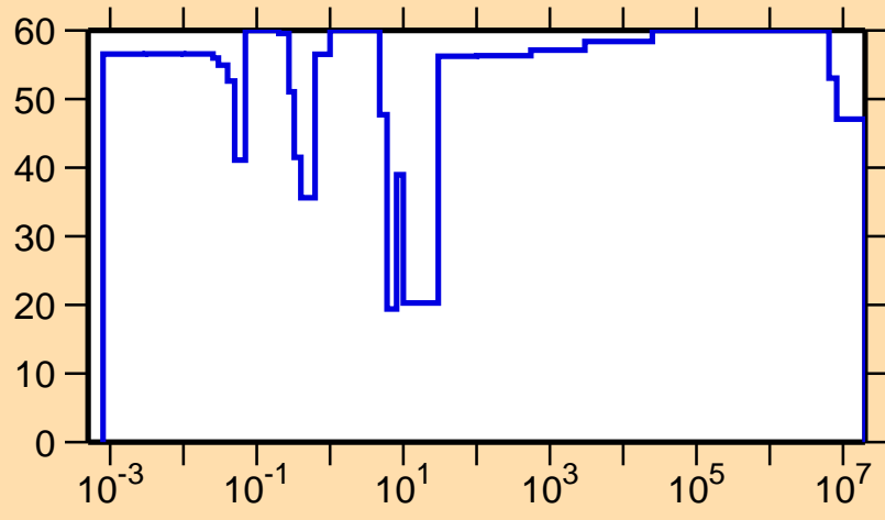
\Delta\sigma/\sigma vs. E for ^{244}\text{Am}(n,\gamma)
