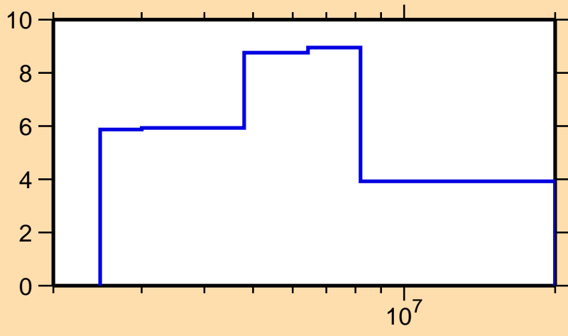
\Delta\sigma/\sigma vs. E for ^{244}\text{Am}(n,el.)
