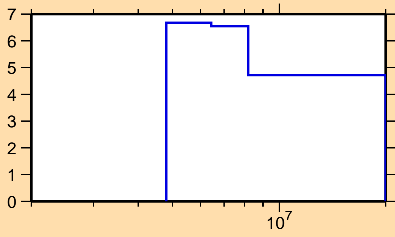
\Delta\sigma/\sigma vs. E for ^{244}\text{Am}(n,\text{tot.})
