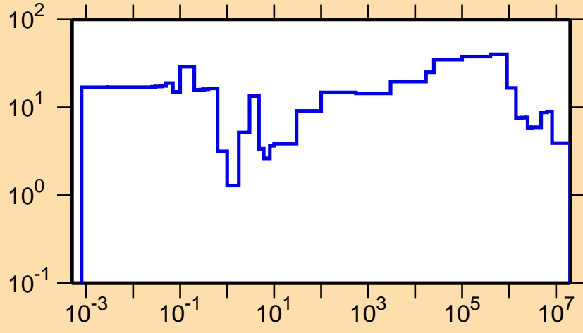
\Delta\sigma/\sigma vs. E for ^{244}\text{Am}(n,el.)
