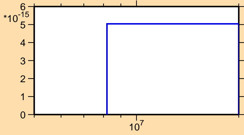
\sigma vs. E for ^{244}\text{Am} (mt 11)
