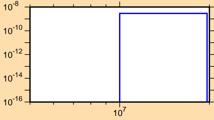
\sigma vs. E for ^{245}\text{Am}(n,2n\alpha)
