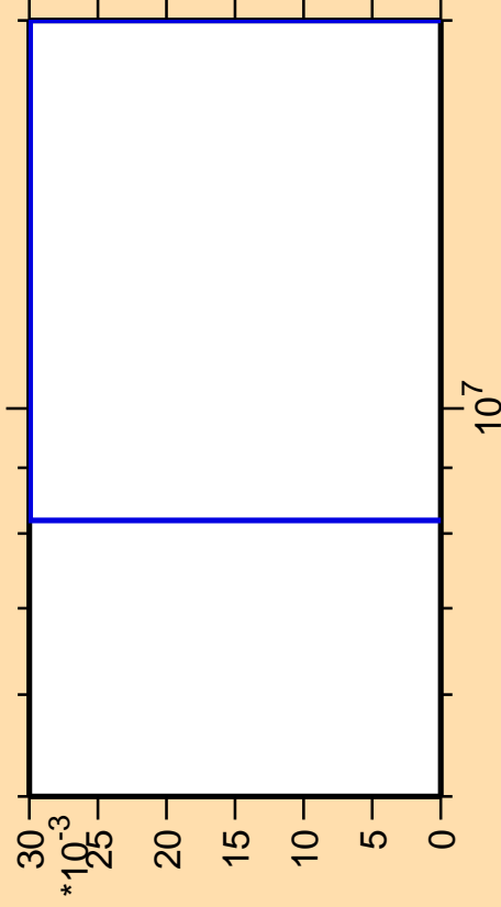
\Delta\sigma/\sigma vs. E for ^{245}\text{Am}(\text{mt } 11)
