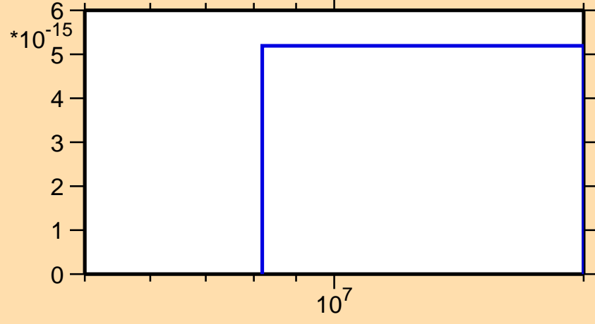
\sigma vs. E for ^{245}\text{Am}(\text{mt } 11)
