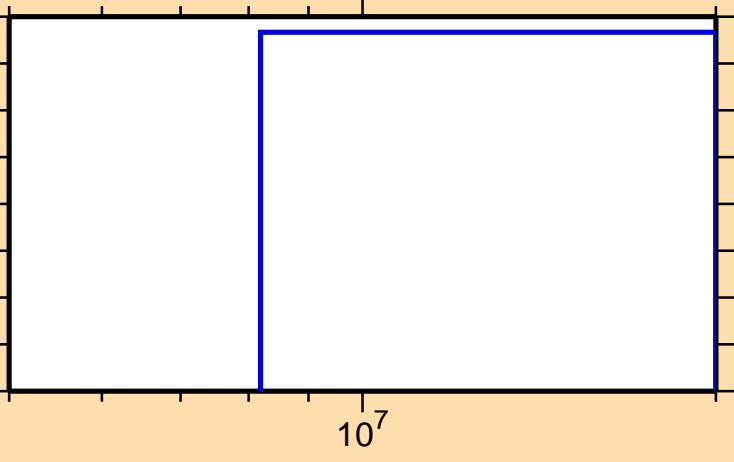
\sigma vs. E for ^{245}\text{Am}(n,\text{nd})
