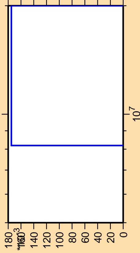
\Delta\sigma/\sigma vs. E for ^{245}\text{Am}(n,3n\alpha)
