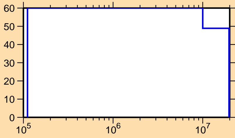
\Delta\sigma/\sigma vs. E for ^{246}\text{Am}(n,n_1)
