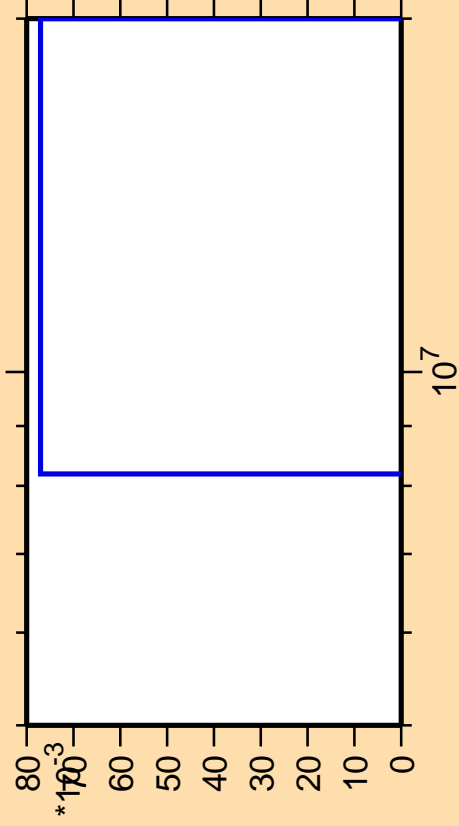
\Delta\sigma/\sigma vs. E for ^{246}\text{Am}(\text{mt } 11)
