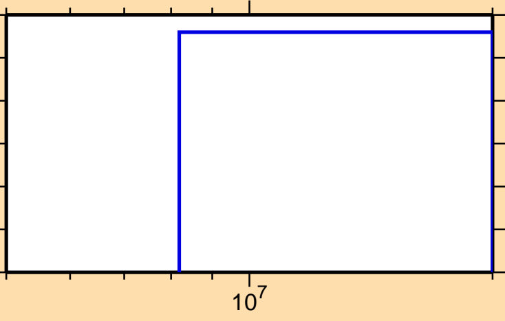
\sigma vs. E for ^{246}\text{Am}(n,np)
