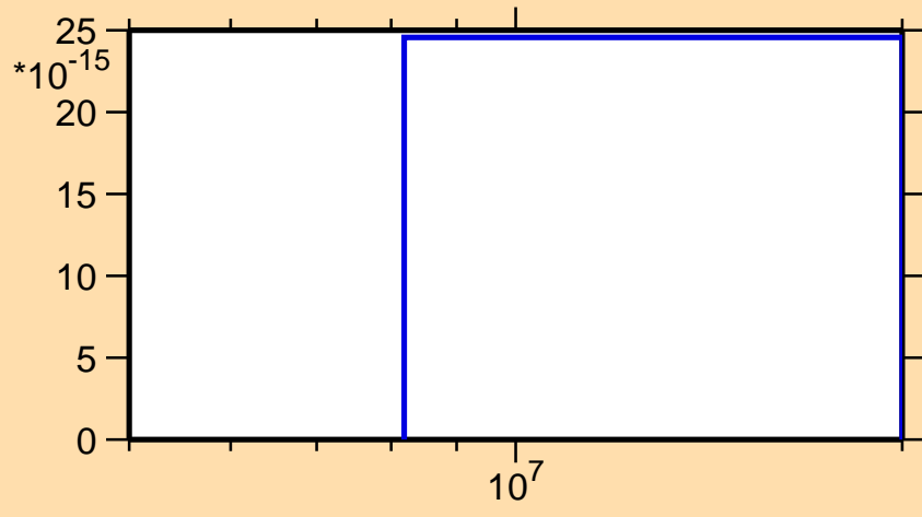
\sigma vs. E for ^{246}\text{Am}(\text{mt } 11)
