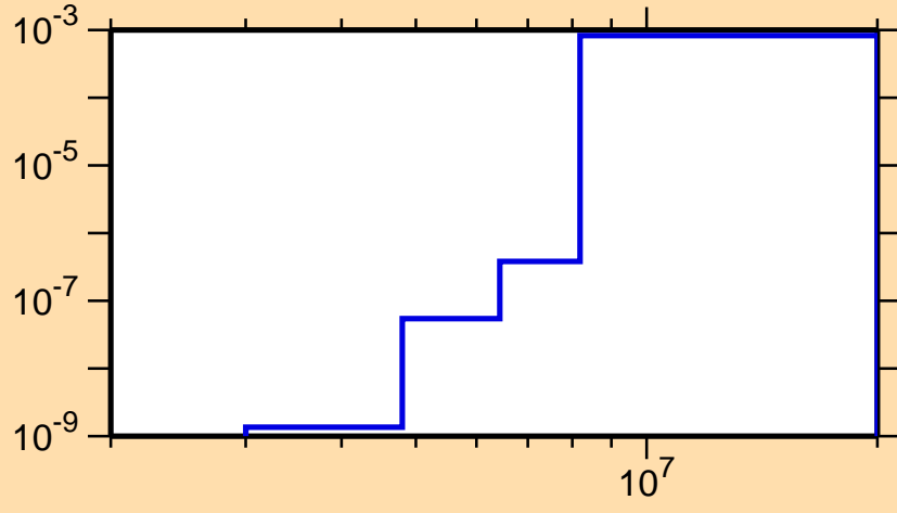
\sigma vs. E for ^{246}\text{Am}(n,n\alpha)
