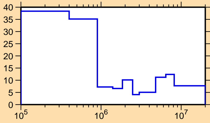
\Delta\sigma/\sigma vs. E for ^{246}\text{Am}(n,\text{tot.})
