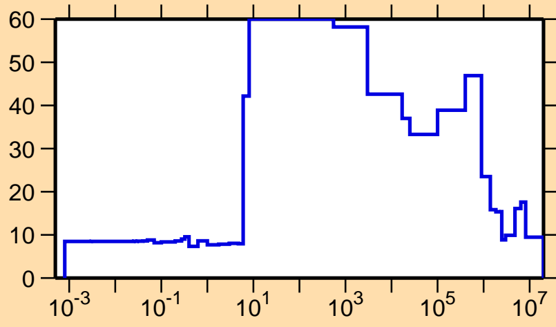
\Delta\sigma/\sigma vs. E for ^{246}\text{Am}(n,el.)
