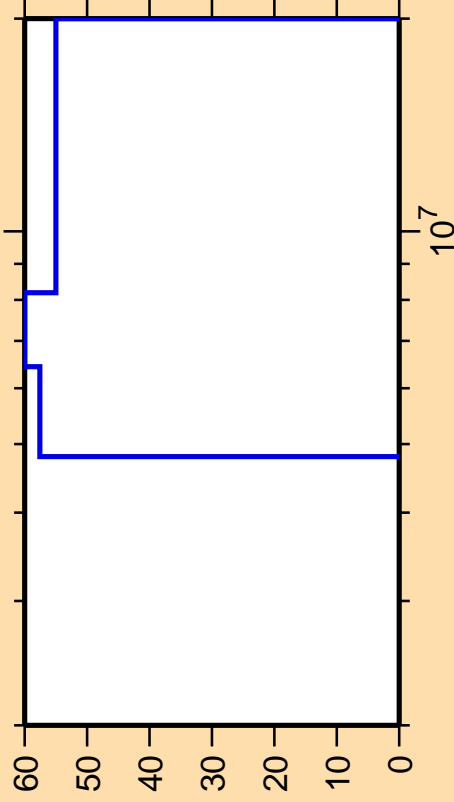
\Delta\sigma/\sigma vs. E for ^{246}\text{Am}(n,n\text{cont.})
