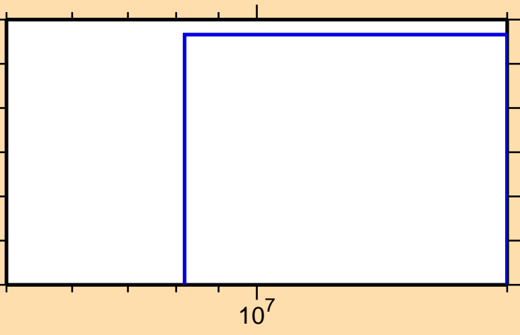
\sigma vs. E for ^{246}\text{Am}(n,nt)
