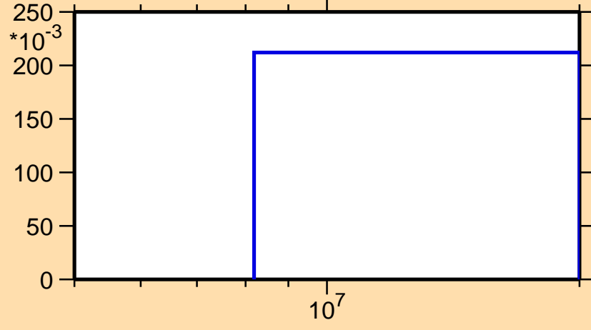
\sigma vs. E for ^{247}\text{Am}(n,3n)
