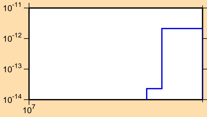
\sigma vs. E for ^{248}\text{Am}(n,\text{He3})
