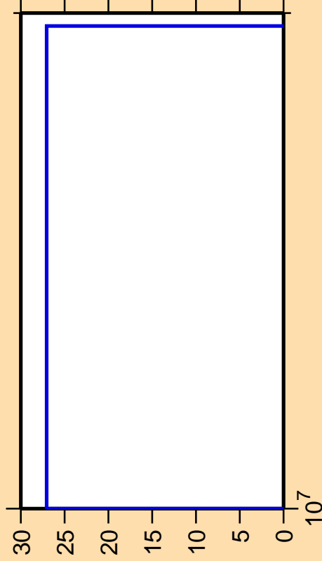
\Delta\sigma/\sigma vs. E for ^{248}\text{Am}(n,\text{nd})
