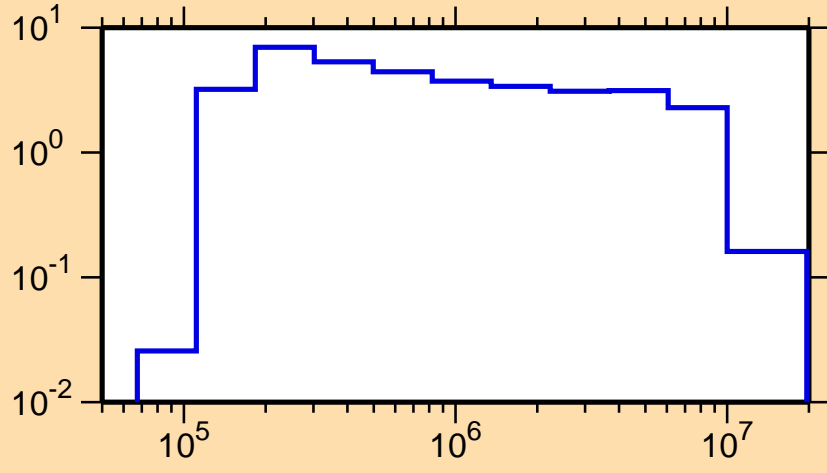
\sigma vs. E for ^{248}\text{Am}(n,n\text{cont.})
