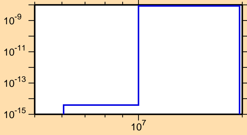
\sigma vs. E for ^{248}\text{Am}(n,2n\alpha)
