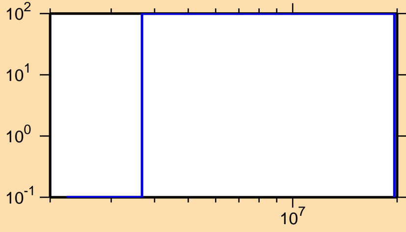
\Delta\sigma/\sigma vs. E for ^{248}\text{Am}(n,p)
