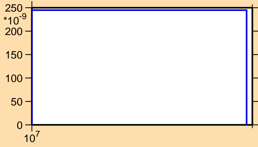
\sigma vs. E for ^{248}\text{Am}(n,\text{nd})
