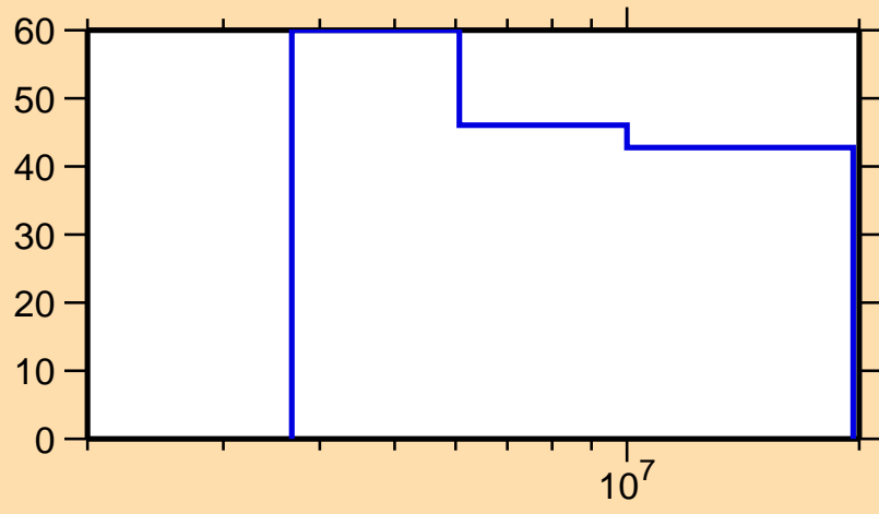
\Delta\sigma/\sigma vs. E for ^{248}\text{Am}(n,2n)
