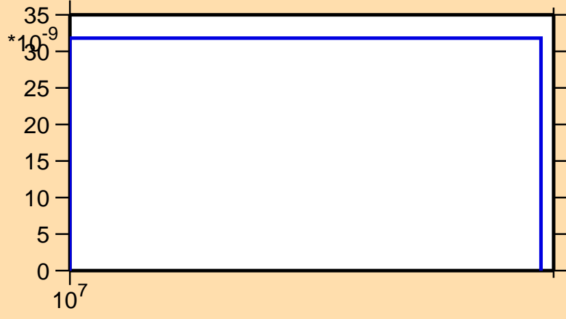
\sigma vs. E for ^{248}\text{Am}(n,2np)
