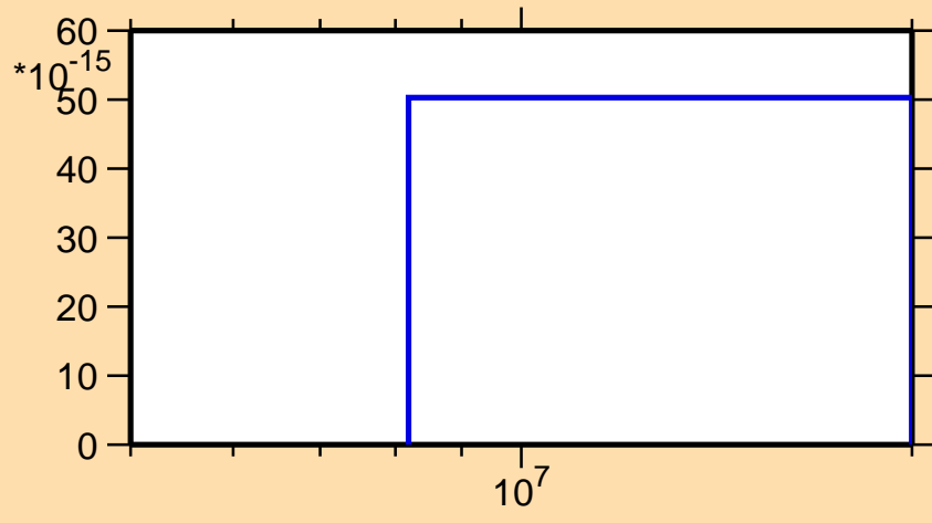
\sigma vs. E for ^{248}\text{Am}(\text{mt } 11)
