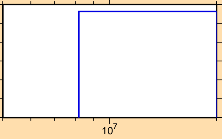
\sigma vs. E for ^{248}\text{Am}(n,np)
