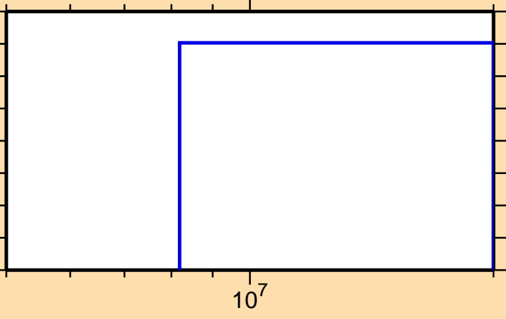
\sigma vs. E for ^{248}\text{Am}(n,2n\alpha)
