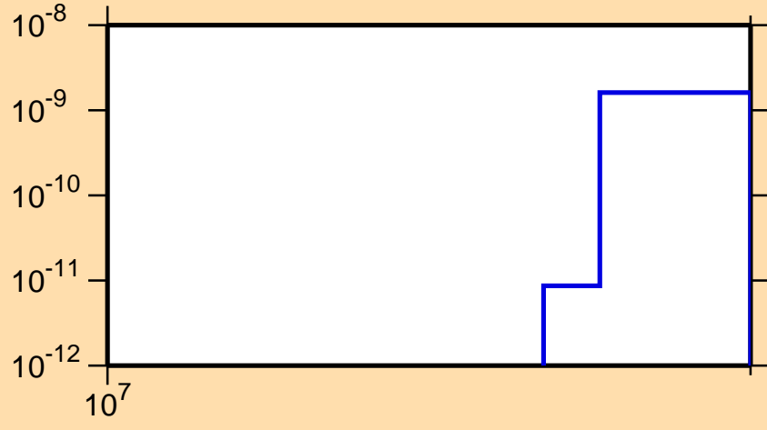
\sigma vs. E for ^{249}\text{Am}(n,3n\alpha)
