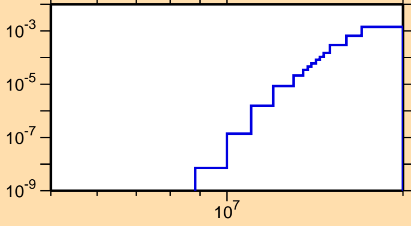
\sigma vs. E for ^{249}\text{Am}(n,t)
