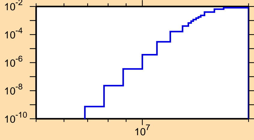
\sigma vs. E for ^{249}\text{Am}(n,\alpha)
