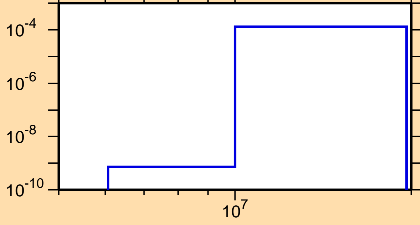
\sigma vs. E for ^{249}\text{Am}(n,t)
