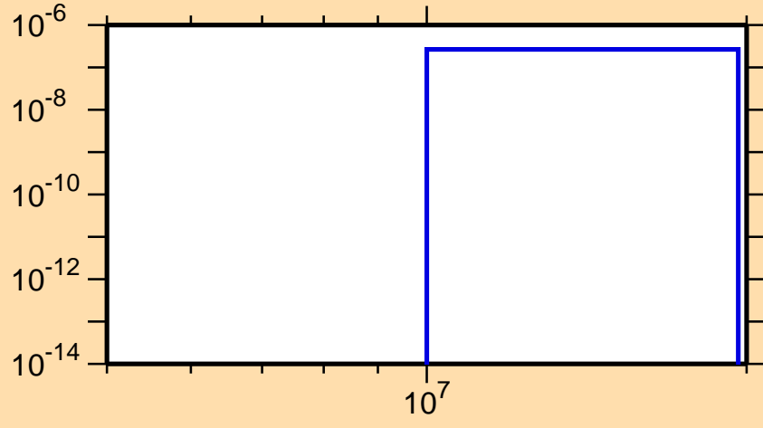
\sigma vs. E for ^{249}\text{Am}(n,2n\alpha)
