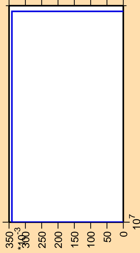
\Delta\sigma/\sigma vs. E for ^{249}\text{Am} (mt 11)
