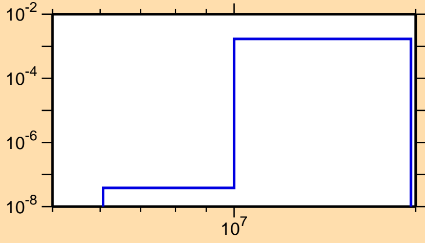
\sigma vs. E for ^{249}\text{Am}(n,\alpha)
