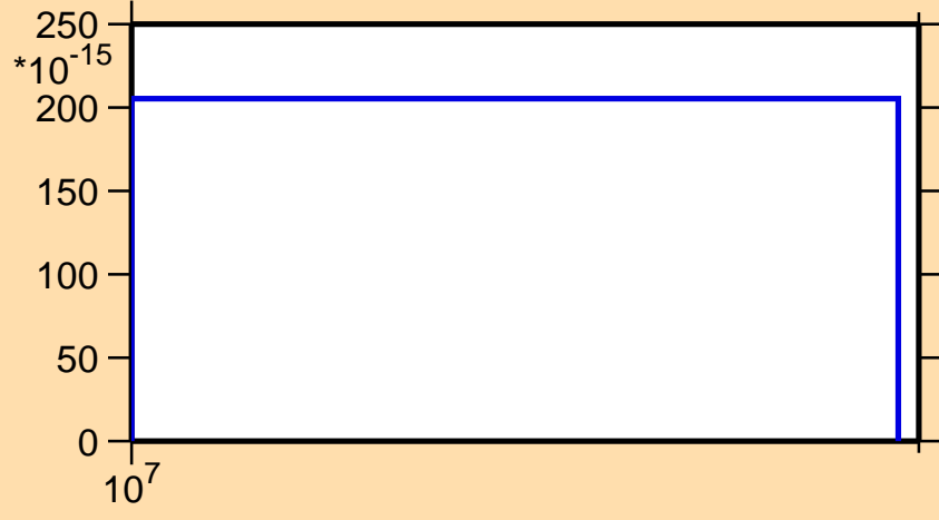
\sigma vs. E for ^{249}\text{Am} (mt 11)
