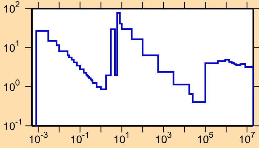
\sigma vs. E for ^{249}\text{Am}(n,\text{nonel.})
