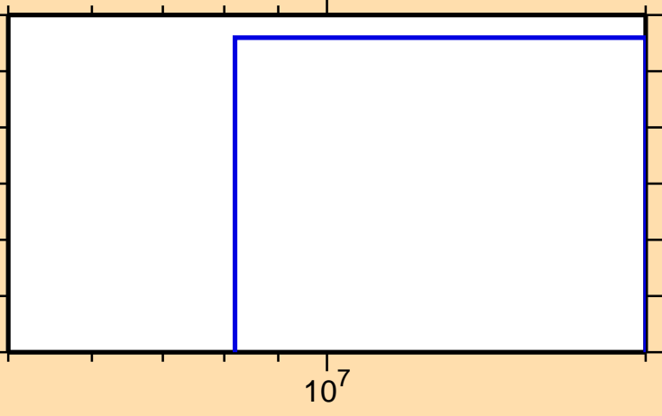
\sigma vs. E for ^{249}\text{Am}(n,nt)
