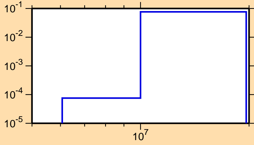
\sigma vs. E for ^{36}\text{Ar}(n,n\alpha)
