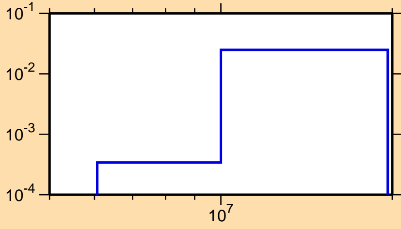
\sigma vs. E for ^{36}\text{Ar}(n,d)
