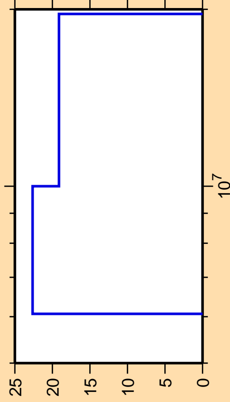
\Delta\sigma/\sigma vs. E for ^{36}\text{Ar}(n,n\alpha)
