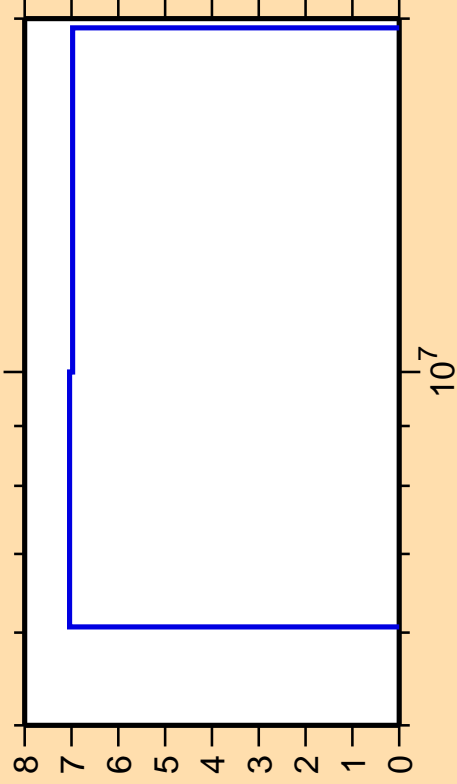
\Delta\sigma/\sigma vs. E for ^{37}\text{Ar}(n,p)
