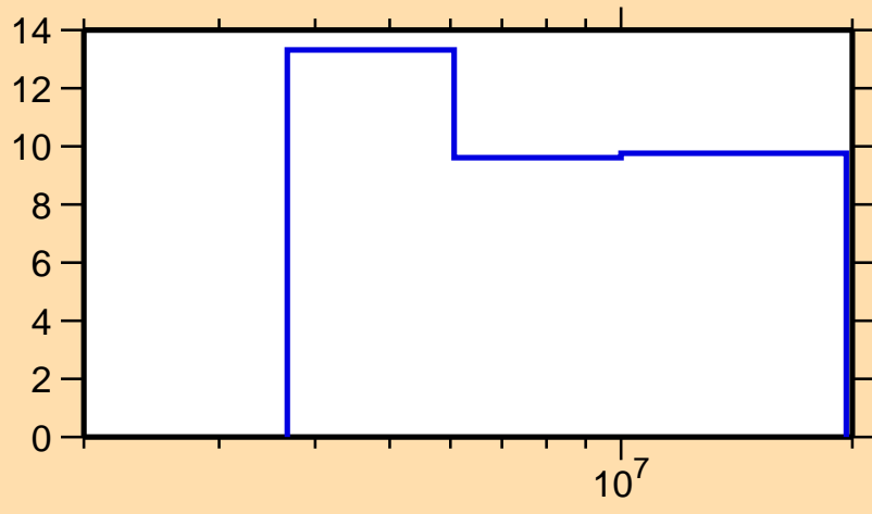
\Delta\sigma/\sigma vs. E for ^{37}\text{Ar}(n,ncont.)
