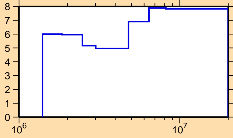
\Delta\sigma/\sigma vs. E for ^{37}\text{Ar}(n,\text{inel.})
