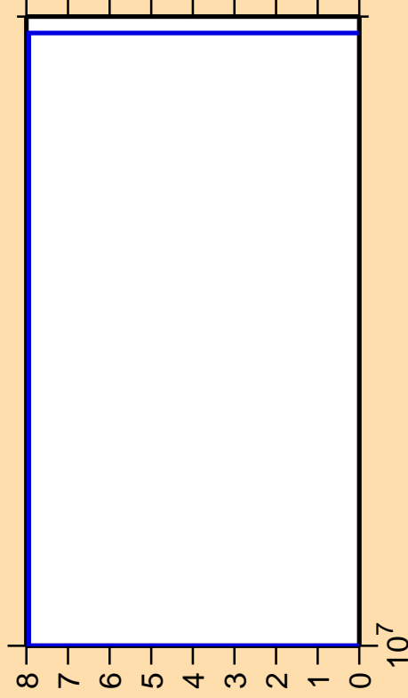
\Delta\sigma/\sigma vs. E for ^{38}\text{Ar}(n,nd)
