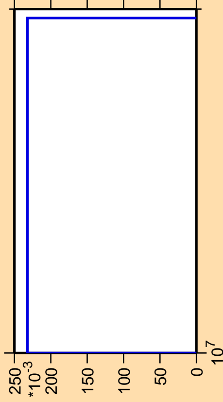
\Delta\sigma/\sigma vs. E for ^{38}\text{Ar} (mt117)
