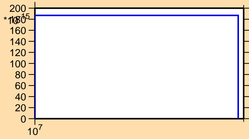
\sigma vs. E for ^{38}\text{Ar} (mt117)
