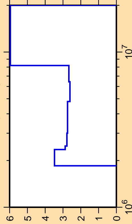
\Delta\sigma/\sigma vs. E for ^{38}\text{Ar}(n,\text{inel.})
