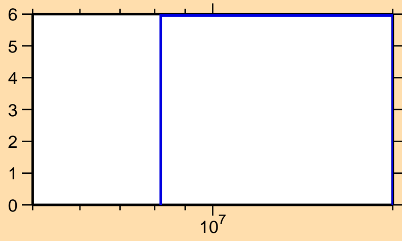
\Delta\sigma/\sigma vs. E for ^{38}\text{Ar}(n,\text{inel.})
