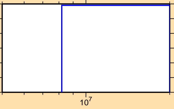
\sigma vs. E for ^{38}\text{Ar}(n,t)
