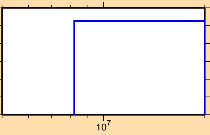
\sigma vs. E for ^{38}\text{Ar} (mt 45)
