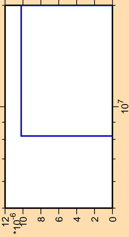
\Delta\sigma/\sigma vs. E for ^{38}\text{Ar} (mt 45)
