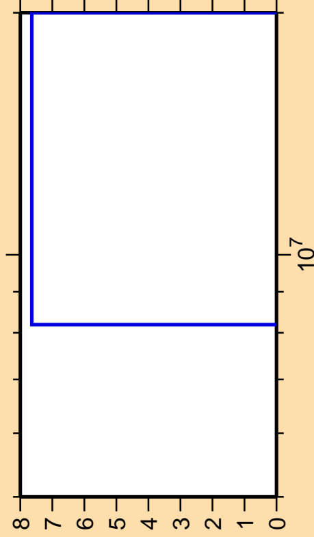
\Delta\sigma/\sigma vs. E for ^{38}\text{Ar}(n,\text{nd})
