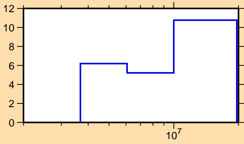
\Delta\sigma/\sigma vs. E for ^{39}\text{Ar}(n,ncont.)
