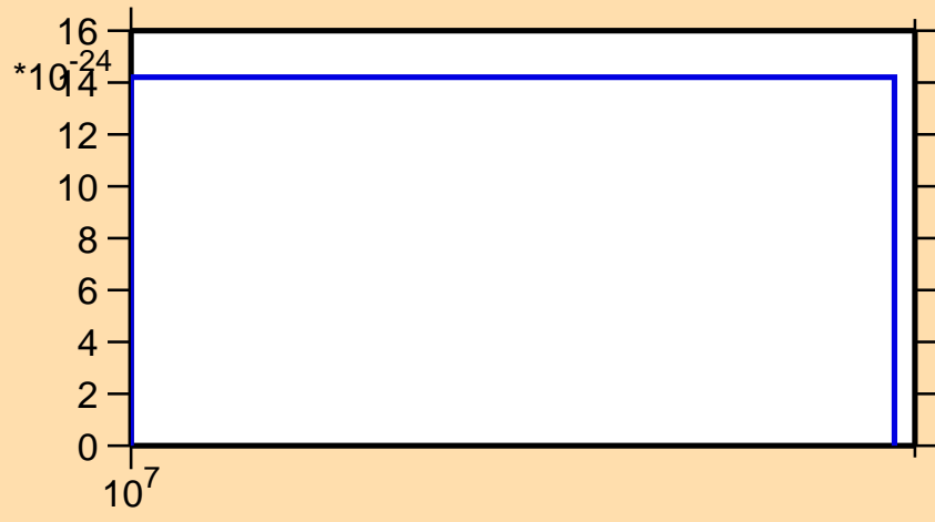
\sigma vs. E for ^{39}\text{Ar} (mt 45)
