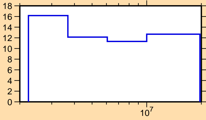
\Delta\sigma/\sigma vs. E for ^{39}\text{Ar}(n,p)
