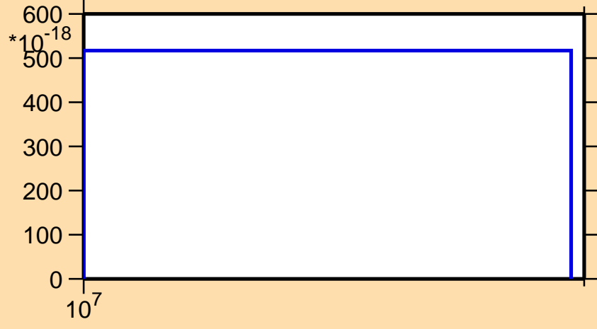
\sigma vs. E for ^{39}\text{Ar} (mt 34)
