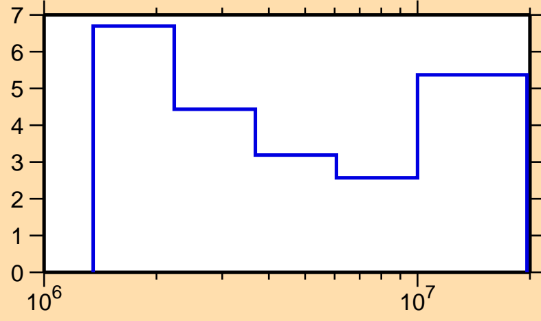
\Delta\sigma/\sigma vs. E for ^{40}\text{Ar}(n,\text{inel.})
