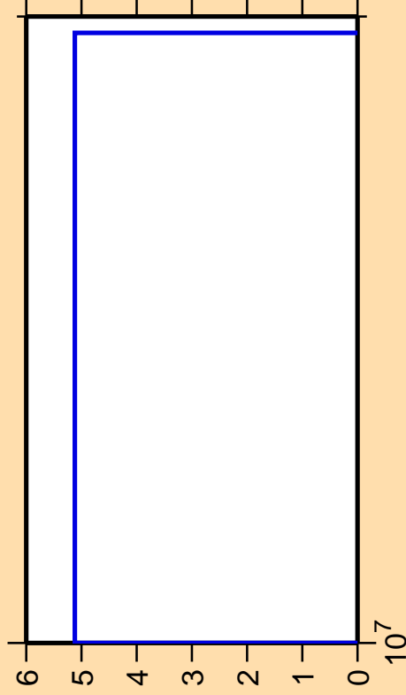
\Delta\sigma/\sigma vs. E for ^{40}\text{Ar}(n,2n\alpha)
