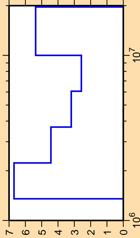
\Delta\sigma/\sigma vs. E for ^{40}\text{Ar}(n,\text{inel.})
