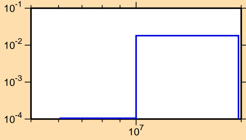
\sigma vs. E for ^{40}\text{Ar}(n,p)
