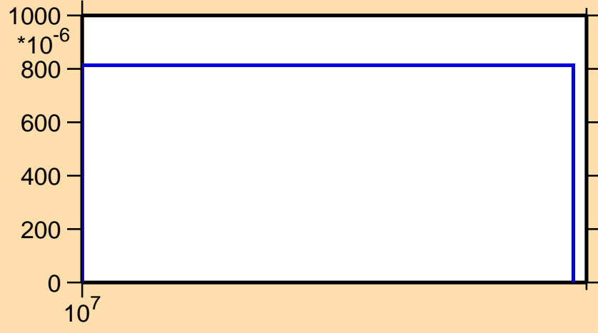
\sigma vs. E for ^{40}\text{Ar}(n,np)
