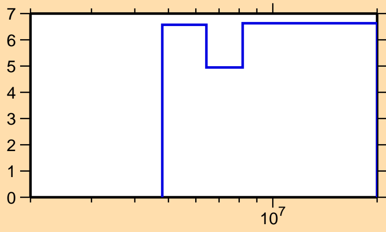
\Delta\sigma/\sigma vs. E for ^{40}\text{Ar}(n,n\text{cont.})
