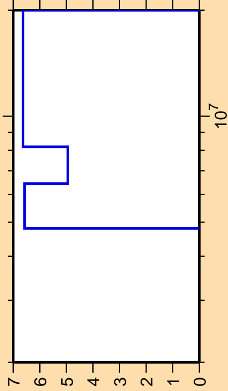
\Delta\sigma/\sigma vs. E for ^{40}\text{Ar}(n,n\text{cont.})
