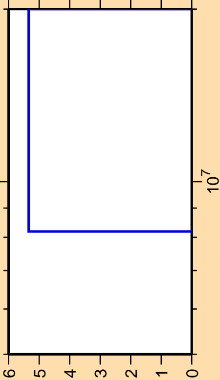
\Delta\sigma/\sigma vs. E for ^{40}\text{Ar}(n,2n)
